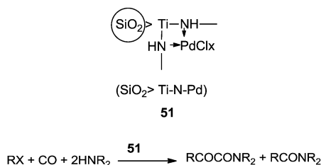
Scheme 63 Reagents and conditions: 51 /PhI (0.5%), phenyl halide (5.1 mmol), \text{Et}_2\text{NH} (100 mmol), temp. 100^\circ\text{C} , CO pressure (3.0 MPa), time 6–24 h.
