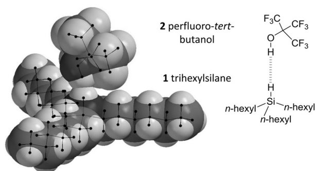
Fig. 3 Minimised geometry of the perfluoro- tert -butanol ( 2 ) and trihexylsilane ( 1 ) complex showing overlap of the van der Waals radii of hydrogen atoms involved in the Si–H \cdots HO interaction. Geometry data for the complex shown (calculated using B3LYP/cc-pVTZ) and those for other theory/basis set combinations are provided in the ESI \ddagger .
