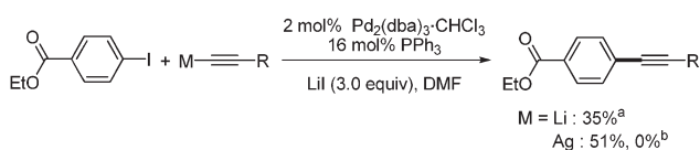
Scheme 6 Decarboxylative coupling with metal phenylacetylides. a THF as solvent; b absence of Lil.
