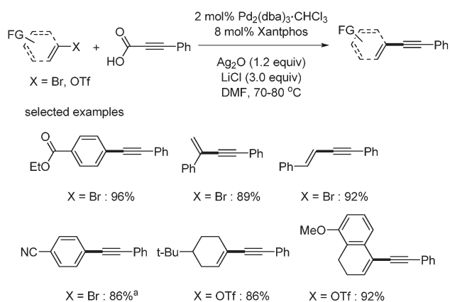
Scheme 5 Decarboxylative coupling with aryl and vinyl bromides and triflates. a Lil was used.
