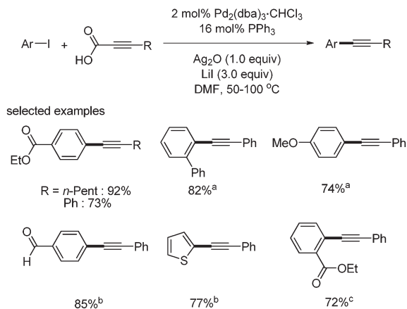
Scheme 4 Decarboxylative coupling with aryl iodides, a 2 equiv. of Ag 2 O, 2 equiv. of phenylpropionic acid and 6 equiv. of Lil were used, b 8 mol% of Xantphos as a ligand, c 1.5 equiv. of Ag 2 O and phenylpropionic acid were used.
