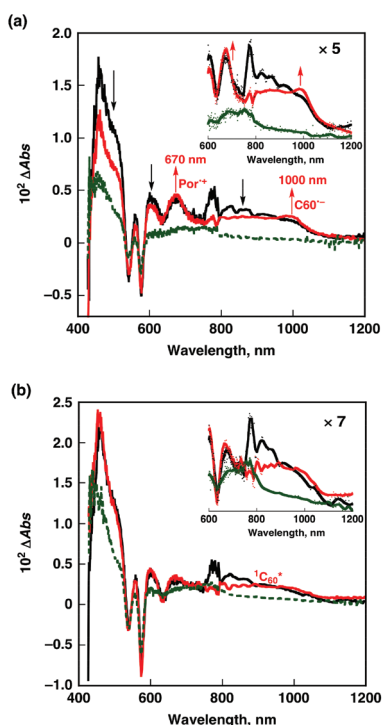
Fig. 13 Transient absorption spectra of (a) \text{TPZn}_3 ( 7.0 \times 10^{-6} \text{ M} ) and (b) MPZn ( 1.1 \times 10^{-5} \text{ M} ) in the presence of \text{PyC}_{60} ( 2.3 \times 10^{-5} \text{ M} ) obtained at 2 ps (black), 62 ps (red), and 2800 ps (green) after femtosecond laser pulse irradiation at 410 nm in deaerated toluene at 298 K.
