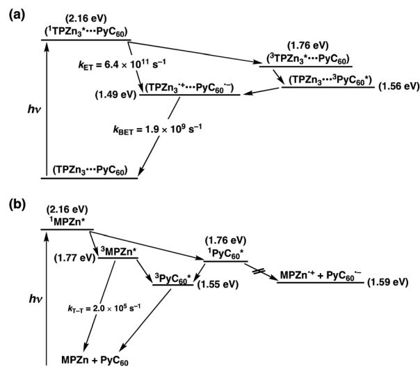
Scheme 4 Energy diagrams for photodynamics of (a) \text{TPZn}_3 and (b) MPZn in the presence of \text{PyC}_{60} in toluene.
