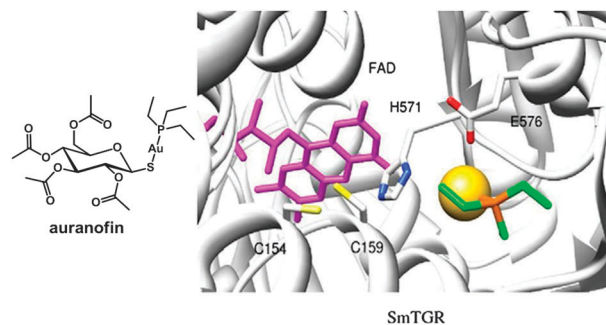
Fig. 11 Molecular structure of auranofin. Docked conformation of {Au(PEt 3 ) + truncated SmTGR. FAD is in violet sticks. The gold atom is a yellow sphere. Residues interacting with the gold atom are in sticks. Adapted from ref. 364.
