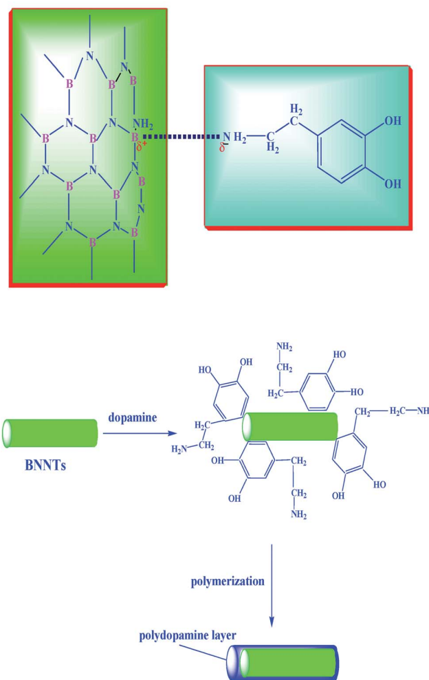
Scheme 1 Schematic illustration of dopamine functionalization of BNNTs.
