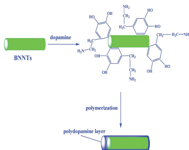
Scheme 1 Schematic illustration of dopamine functionalization of BNNTs.
