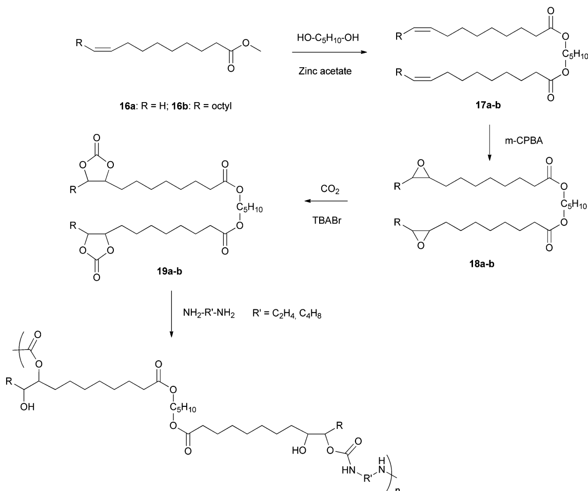
Scheme 10 Polyurethane from methyleates.
