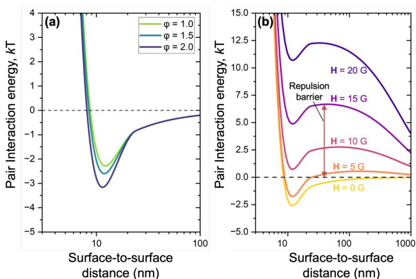
Figure 2. (a) Total pair interaction potentials plotted for varying MNPs concentration ( \phi – vol %) at \mathbf{H} = 2.5 G, increasing \phi leads to the appearance of attraction well causing PS microspheres to assemble. (b) Total pair interaction potentials plotted for varying \mathbf{H} with constant ( \phi = 1.5 vol %). The repulsion barrier formed at large \mathbf{H} prevents the PS microspheres from assembling.
