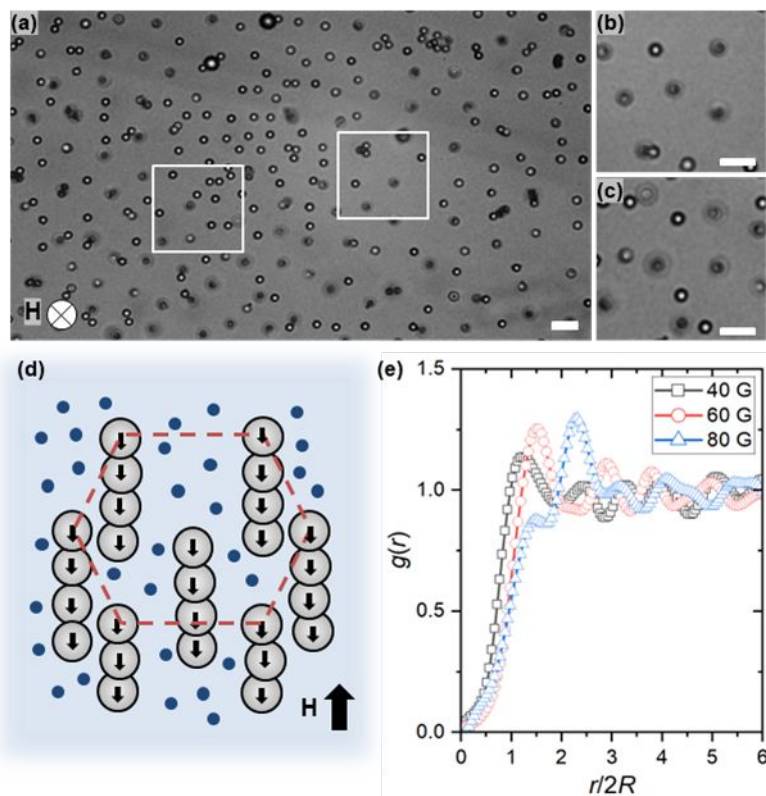
Figure 4. (a) Microscope image of Wigner glass structures observed at \mathbf{H} = 80 G. (b-c) Magnified views of the boxed regions showing the formation of chains of PS microspheres orthogonal to the viewing plane. Scale bars in (a-c) are 5 \mu\text{m} . (d) Schematic of PS microspheres forming out-of-plane chains in the presence of magnetic field \mathbf{H} . Red dashed lines indicate particles ordering in a hexagonal arrangement. (e) Radial distribution function g(r) in a 2D plane for \mathbf{H} = 40 G, 60 G, and 80 G. The separation distance is normalized with particle diameter ( 2R ).
