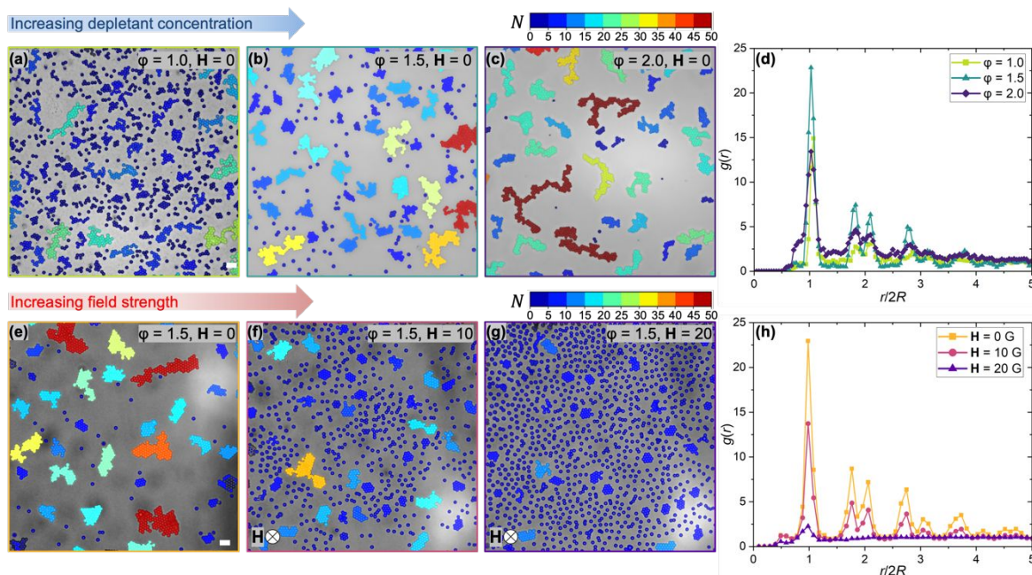
Figure 3. (a-c) Images captured for equilibrium structures obtained at \phi = 1.0, 1.5, and 2.0 vol %, respectively, in the absence of an external magnetic field. The images illustrate the transition from discrete 2D clusters to large 3D fractal clusters. (d) Radial distribution function g(r) in a 2D plane for varying \phi in the absence of magnetic field \mathbf{H} . (e-g) Images captured for structures obtained at magnetic field strength, \mathbf{H} = 0, 10, 20 G, and fixed MNPs concentration ( \phi = 1.5 vol %). Scale bars in a and e are 5 \mu\text{m} . (h) Radial distribution function g(r) in a 2D plane for varying \mathbf{H} at constant \phi = 1.5 vol %.
