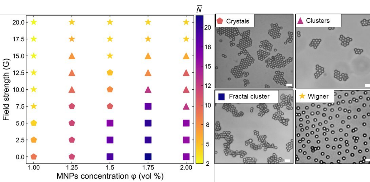
Figure 5. Phase diagram for colloids interacting via competing d-SALR interactions based on the average number of particles in a structure ( \bar{N} ). Symbols indicate different structures: Colloidal 2D crystals (pentagon), 2D clusters (triangles), fractal clusters (squares), and Wigner glass (stars), as shown by the images on the right. The color of the individual symbol represents the average number of particles ( \bar{N} ) within the assembled structure.
