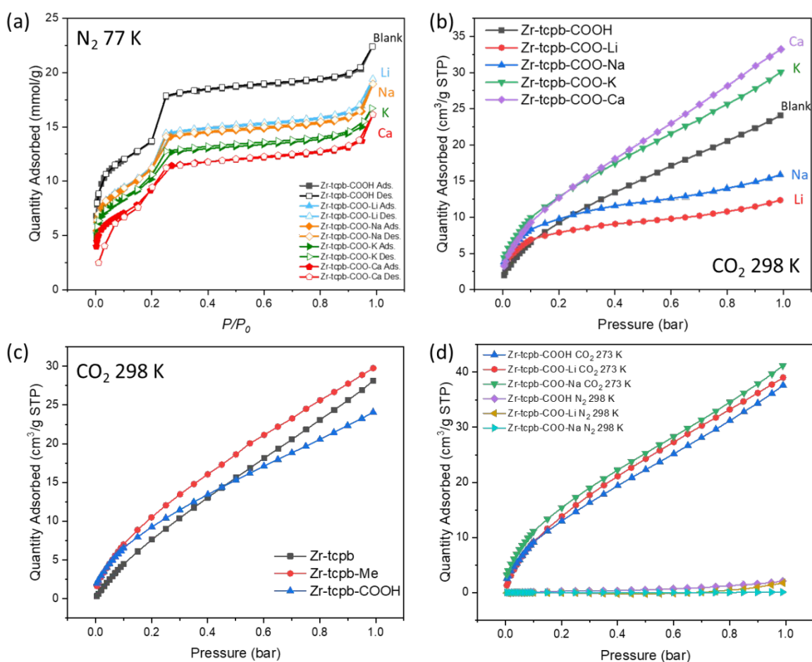
Figure 3. The gas adsorption-desorption isotherms of Zr-tcpb-COOM: (a) \text{N}_2 at 77 K and (b) \text{CO}_2 at 298 K; (c) The \text{CO}_2 adsorption isotherms of un-modified Zr-tcpb-X at 298 K; (d) Comparisons of adsorption isotherms of \text{CO}_2 and \text{N}_2 at 273 K and 298 K.
