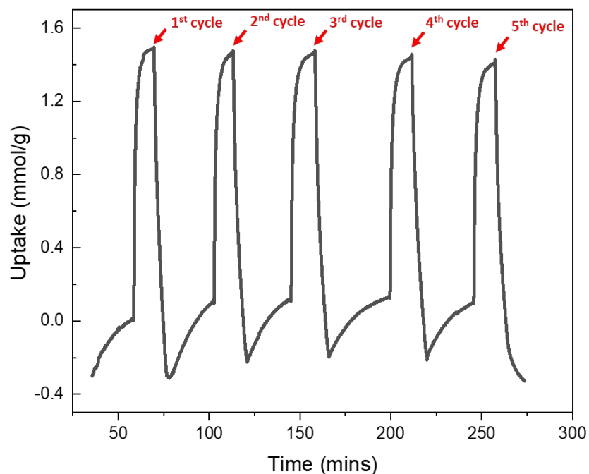
Figure 5. The CO 2 adsorption-desorption recyclability test results for the Zr-tcpb-COOCa sample. Five consecutive adsorption cycles were carried out with a gas feeding ratio CO 2 : N 2 = 95:5 (v:v) at 303 K.
