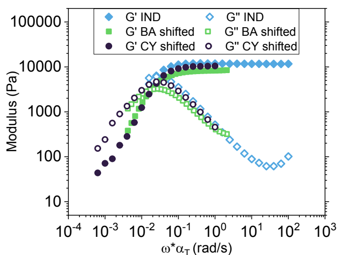
Figure 4. Time—cross-linker superposition for both the storage ( G' ) and loss ( G'' ) moduli of networks with three different cross-linkers ( IND , BA , and CY ). IND was used as the reference.
