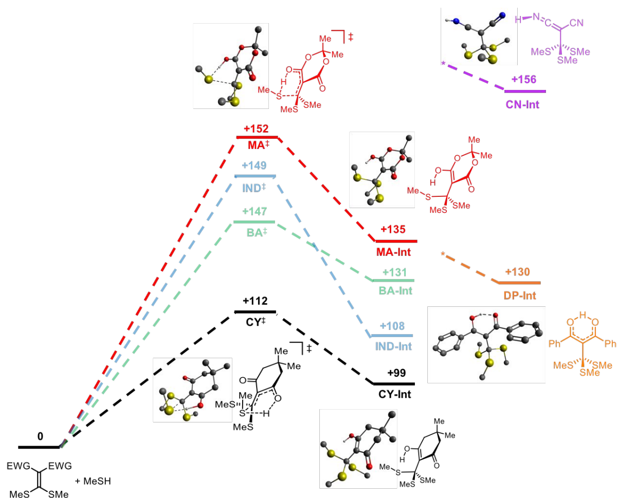
Figure 2. Calculated transition states and intermediate energies for the cross-linkers (energies are not drawn to scale). Representative optimized cyclic transition state and intermediates for the conjugate addition of methanethiol to MA and CY, and intermediates for CN and DP, are shown. H atoms on CH 3 groups are omitted for clarity. *No cyclic transition states were located for DP and CN.
