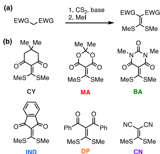
Figure 1. (a) General synthesis for cross-linkers used in the study. (b) Structures of different cross-linkers used in the study.
