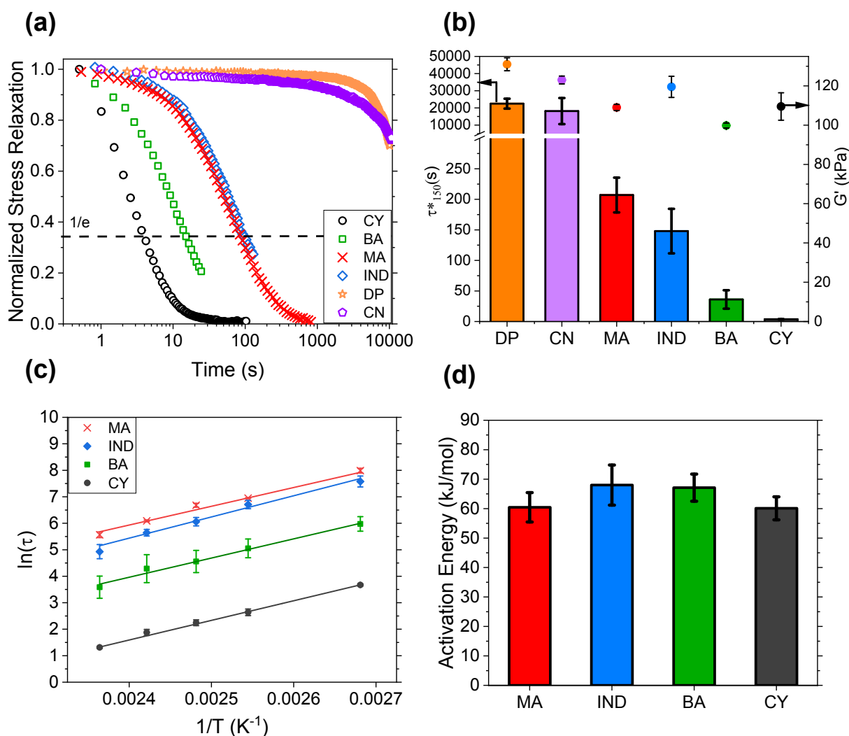
Figure 3. Mechanical properties of the networks. (a) Representative normalized stress relaxation profiles at 150 °C. (b) Calculated \tau^* values for the different cross-linked vitrimers (bar graph, left axis) and their rubbery plateau moduli at the same temperature (circle symbols, right axis). Error bars are based on student's t distribution. The \tau^* values calculated using 1/e of the relaxation modulus for the cyclic cross-linkers and by extrapolating a stretched exponential function for the acyclic cross-linkers (see ESI for more detail). (c) Arrhenius plots for stress relaxation of networks derived from the cyclic cross-linkers. (d) Calculated flow activation energies for the networks. Error bars are based on the error analysis of the fitted slopes.
