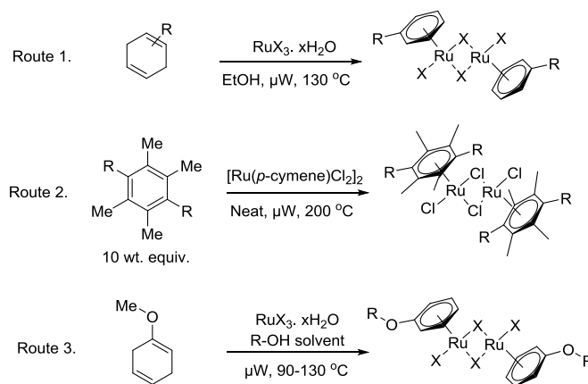
Figure 2: Synthetic routes for the formation of aryl ruthenium halide dimers
