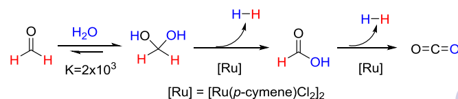
Figure 1: Ruthenium catalysed hydrogen release from aqueous formaldehyde
