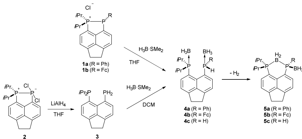
Scheme 1: Synthesis of bis(borane) adducts 4a–c and \text{BH}_2 bridged compounds 5a–c .
