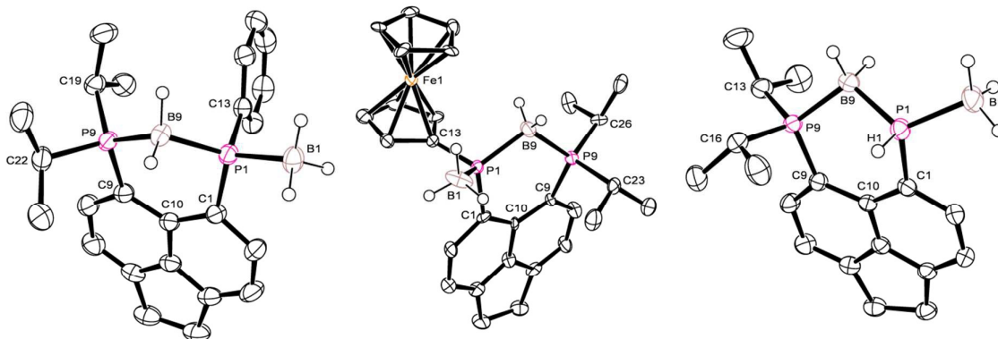
Figure 5: Structures of 5a (left), 5b (centre), and 5c (right) in the solid state. Carbon-bound hydrogen atoms and second molecule in asymmetric unit (for 5b and 5c ) omitted for clarity.
