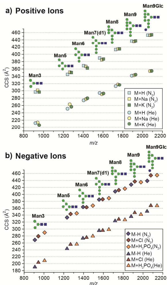
Figure 1: Absolute collision cross sections ( ^{DT}CCS ) of N-glycan standards measured in nitrogen and helium as [M+H]^+ , [M+Na]^+ , [M+K]^+ , [M-H]^- , [M+Cl]^- and [M+H_2PO_4]^- adducts using drift tube ion mobility-mass spectrometry. For ATDs that exhibit multiple features the most abundant feature was used for CCS determination. Mannose residues are shown in green circles, N-acetylglucosamine residues are blue squares, and glucose residues are blue circles. Glycosidic linkages are based on the Oxford Glycan Nomenclature. 1
