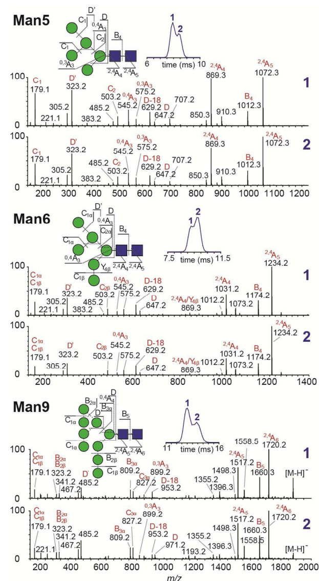
Figure 3: Negative ion MS/MS spectra of synthetically derived Man5, Man6 and Man9 [M-H]^- ions. Fragmentation is identical between ATD peaks 1 and 2 from each sample confirming the presence of a single structure.
