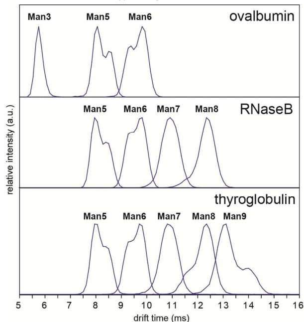
Figure 4: Arrival time distributions of [M-H]^- high-mannose N-glycans from ovalbumin, RNase B and thyroglobulin. The presence of multiple conformers is evident for Man5, Man6 and Man9. Measurements were performed using a TW IM-MS instrument.
