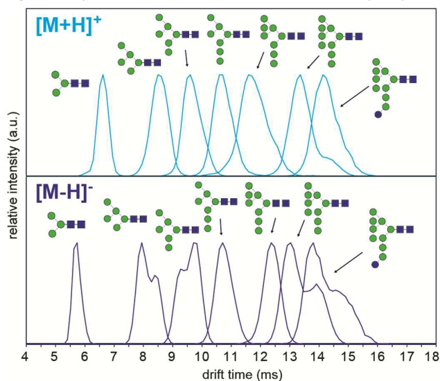
Figure 2: Arrival time distributions (ATDs) of synthetic high-mannose N-glycans as [M-H]^- and [M+H]^+ ions. Multiple features are observed in the ATDs of Man5, Man6, Man9 and Man9Glc [M-H]^- ions, which points to the coexistence of multiple conformers. Measurements were performed using a TW IM-MS instrument.
