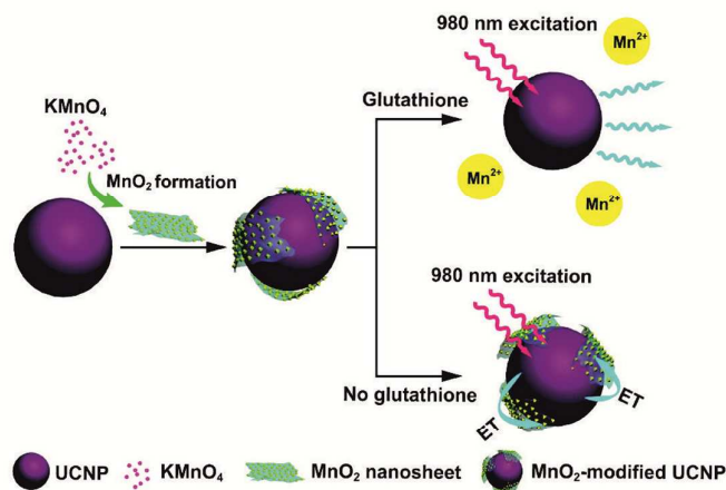
Figure 19 Design and function of a glutathione (GSH) sensitive probe based on UCNPs. The emission of the UCNPs is quenched by the manganese oxide ( \text{MnO}_2 ) nanosheets formed on the nanoparticle surface. The analyte GSH reduces \text{MnO}_2 , removes the nanosheets, and restores the emission of the UCNPs. Reprinted with permission from Ref. 37. Copyright © 2011, American Chemical Society.
