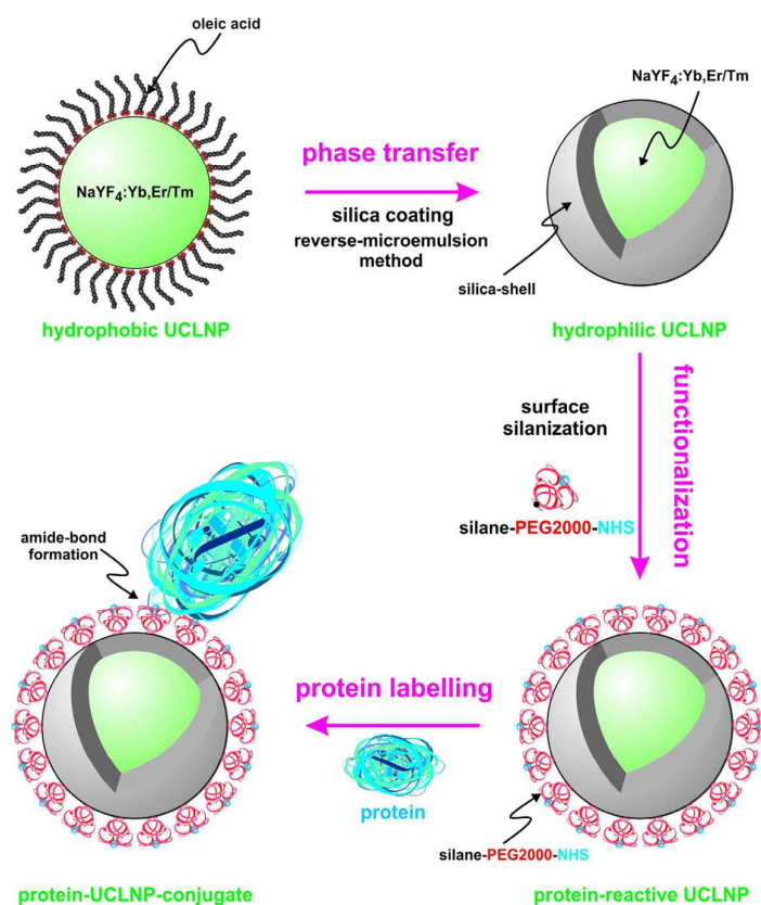
Figure 15 Surface engineering of UC(L)NPs. Silica-coating renders UC(L)NPs water dispersible and provides an attachment site for silanization that can then be used for the covalent attachment of proteins or other biomolecules. Reprinted with permission from Ref. 152 Copyright © 2013, Theranostics.
