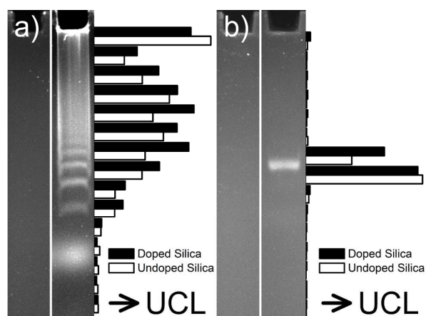
Figure 28 Agarose gel electrophoresis reveals nanoparticle aggregation. (a) UCNPs coated with a bare silica shell are separated in several distinct bands, which can be attributed to discrete clusters of UCNPs. (b) Silica-
