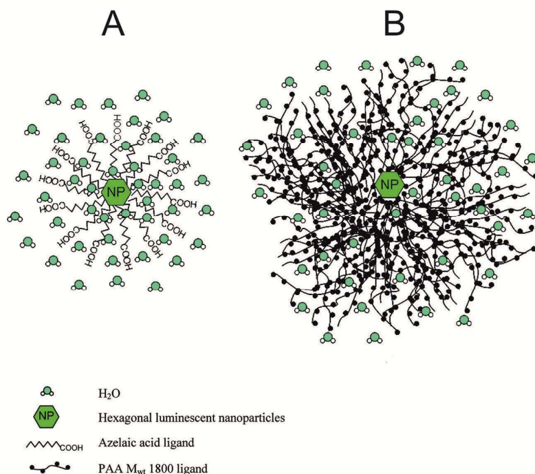
Figure 6 Shielding effect from water molecules of (A) azelaic acid (small/linear ligand) and polyacrylic acid ( M_w = 1800 , large/bulky) resulting in differing quenching factors of the upconversion luminescence by water. Reprinted with permission from Ref. 99. Copyright © 2009, American Chemical Society.
