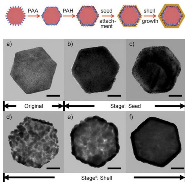
Figure 20 Upper scheme: Surface functionalization, attachment of gold nanoparticles, and growth of a gold nanoshell on an UCNP. Lower TEM images of UCNPs during gold seed attachment and shell growth, a) original, b–c) with increasing number of attached gold nanoparticles and d–f) with growing gold nanoshells (scale bar: 50 nm). Reprinted with permission from Ref. 125 Copyright © 2010, Wiley.
