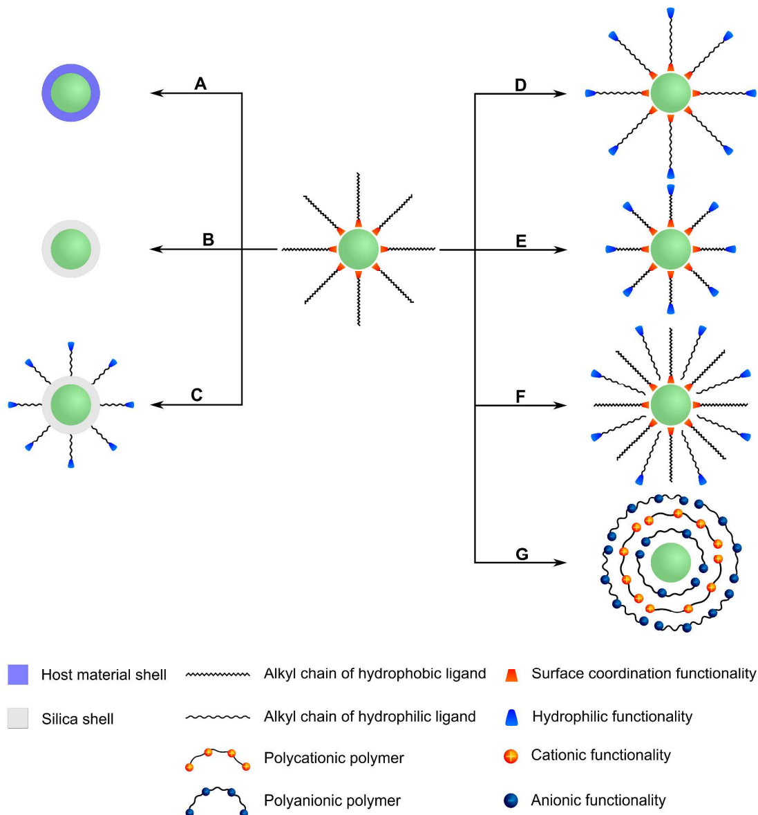
Figure 2 Common routes for the surface modification of oleic acid-coated UCNPs: (A) Surface passivation enhances the upconversion efficiency. (B) A silica shell is chemically inert and confers water dispersibility. (C) Functional groups can be bound covalently to the silica shell by silanization. Oleic acid can be replaced by a ligand exchange reaction (D) or oxidized (E) to yield a hydrophilic surface functionalization. (F) Ligand interactions are exploited to insert further layers of ligands on the surface of UCNPs. (G) Polyanions and polycations can be deposited on the UCNP surface by the layer-by-layer (LbL) technique.
