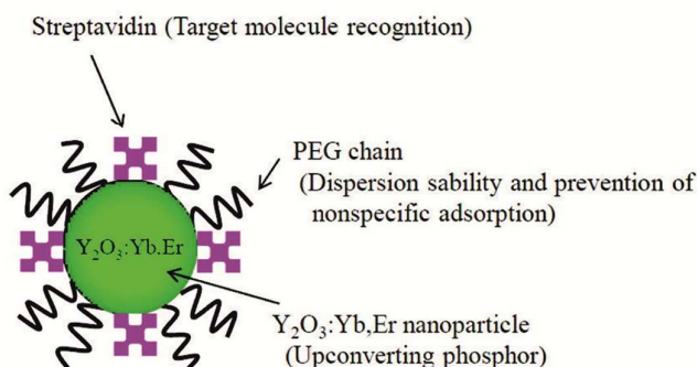
Figure 16 Scheme of UCNPs coated by PEG-PAA and streptavidin by ligand exchange reaction. The polymer increases the dispersion stability and prevents non-specific binding, while streptavidin serves as a binding site for target molecules. Reprinted with permission from Ref. 33. Copyright © 2008, American Chemical Society.
