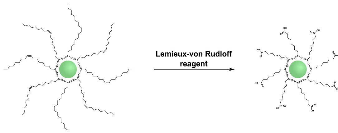
Figure 9 Scheme of the oxidation of oleic acid with the Lemieux-von Rudloff reagent ( \text{MnO}_4^-/\text{IO}_4^- ). The oxidation of the double bond leads to the formation of hydrophilic carboxylate groups on the UCNP surface which are accessible for subsequent conjugation steps. Adapted with permission from Ref. 28. Copyright © 2008, American Chemical Society.
