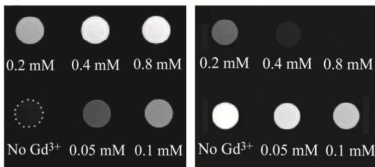
Figure 29 MR images of \text{NaYF}_4@\text{SiO}_2 functionalized with a \text{Gd}^{3+} -coordinating complex with varying gadolinium concentrations (left: T_1 -weighted; right: T_2 -weighted). The reference solution (“No \text{Gd}^{3+} ”) contains the \text{NaYF}_4@\text{SiO}_2 functionalized with the complex but without any coordinated \text{Gd}^{3+} . The \text{Gd}^{3+} -functionalized UCNPs are more applicable for T_1 -weighted MRI. Reprinted with permission from Ref. 147. Copyright © 2009, American Chemical Society.
