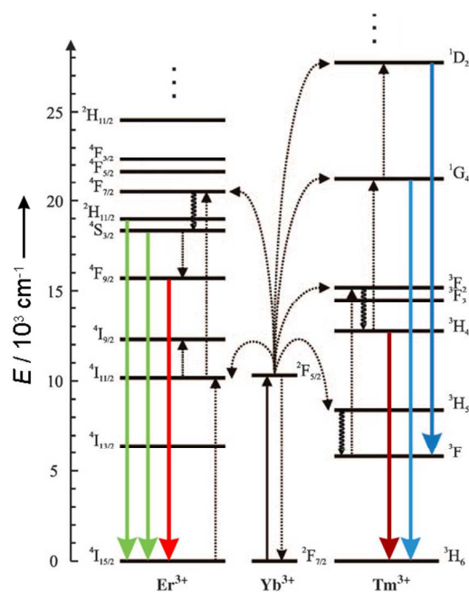
Figure 1 Energy-level diagram of anti-Stokes processes in UCNPs ( \text{NaYF}_4:\text{Yb,Er/Tm} ). The sensitizer ion \text{Yb}^{3+} absorbs NIR light, and the activator ions \text{Er}^{3+} or \text{Tm}^{3+} emit visible or NIR light. Sensitizer and activator ions are embedded in a hexagonal nanocrystal of \text{NaYF}_4 . Full arrows: radiative transitions, dotted arrows: non-radiative energy transfer, curled arrows: multiphonon relaxation. Adapted from Ref. 2 with permission.
