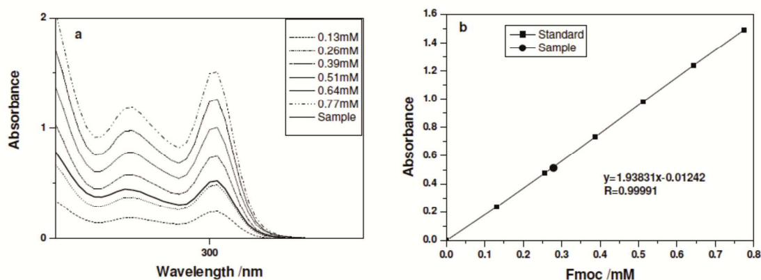
Figure 26 Quantitative analysis of amine groups on the UCNP surface via Fmoc labeling. After labeling the amines bound to the UCNP surface with Fmoc and a washing step to remove excess Fmoc, the Fmoc group is cleaved from the amines. The Fmoc concentration of the sample is determined via UV spectroscopy (left) and the amine content can be calculated using calibration solutions (right). Reprinted with permission from Ref. 122. Copyright © 2011, American Chemical Society.
