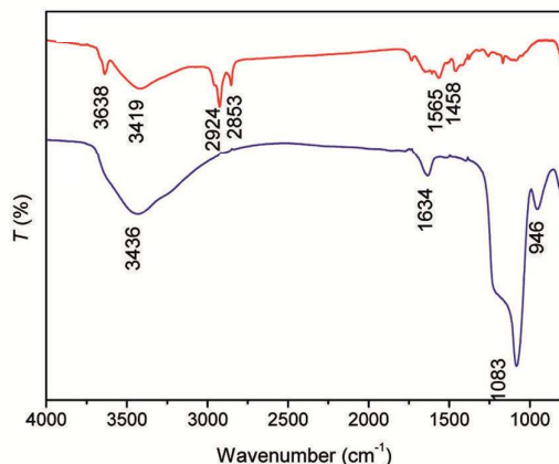
Figure 25 FTIR spectra of unmodified NaYbF 4 : Er UCNPs (upper red curve) and silica-coated NaYbF 4 : Er UCNPs (lower blue curve). The strong new band at 1083 cm -1 is assigned to stretching vibration of Si-O. Reprinted with permission from Ref. 163. Copyright © 2009, American Chemical Society.
