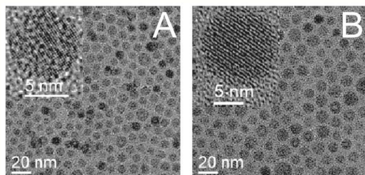
Figure 22 TEM images of (A) core-only NaYF 4 : Yb, Er UCNPs and (B) core/shell UCNPs NaYF 4 : Yb, Er @NaYF 4 . The increase in diameter is attributed to the growth of an undoped host material shell on the surface of the core-only UCNPs. Reprinted with permission from Ref. 70. Copyright © 2007, American Chemical Society.
