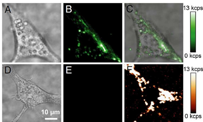
Figure 11 Endocytosis of PAA-coated UCNPs by murine fibroblasts (NIH 3T3). (A) Brightfield image of a cell with endocytosed UCNPs, (B) upconverting luminescence under 980-nm excitation, and (C) overlay. (D) Brightfield image of a cell without UCNPs, (E) upconverted luminescence under 980-nm excitation, and (F) cellular autofluorescence under 532-nm excitation. Reprinted with permission from Ref. 24 Copyright © 2009, PNAS.
