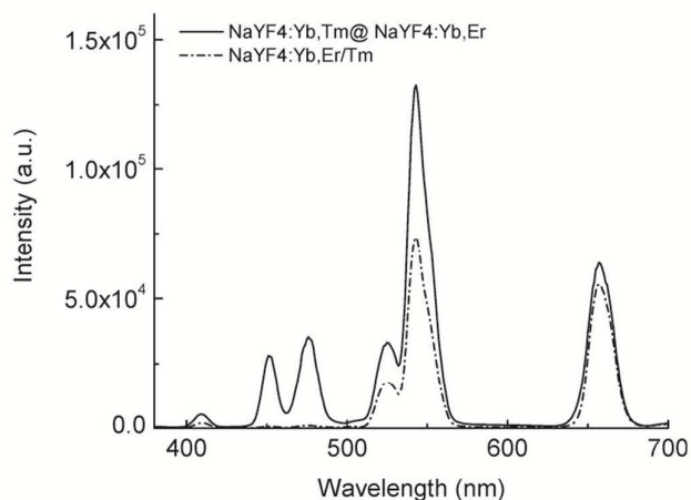
Figure 5 Luminescence spectra of active-core/active-shell \text{NaYF}_4 UCNPs (Emission bands of \text{Tm}^{3+} : 409 nm, 450 nm and 475 nm; emission bands of \text{Er}^{3+} : 520 nm, 541 nm and 653 nm). The spatial separation of the two activators in \text{NaYF}_4:\text{Yb},\text{Tm}@NaYF_4:\text{Yb},\text{Er} avoids quenching of the activators compared co-doped \text{NaYF}_4:\text{Yb},\text{Er}/\text{Tm} UCNPs. Reprinted with permission from Ref. 84. Copyright © 2008, American Chemical Society.
