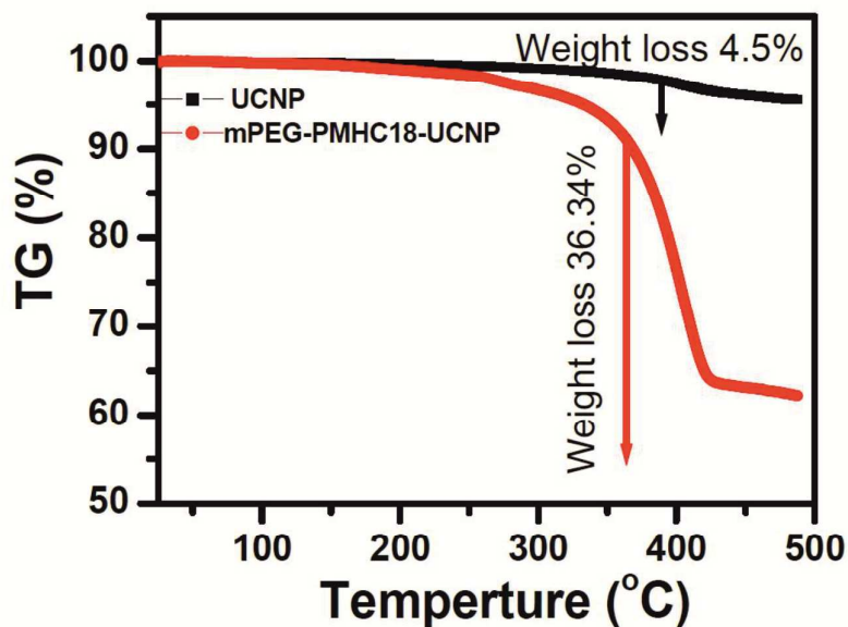
Figure 24 Thermogravimetric analysis (TGA) curves of UCNPs coated with oleic acid (black curve) or PEG-PMHC 18 (red curve). The expected larger weight loss of PEG-coated UCNPs with 36.34 % compared to unmodified UCNPs with only 4.5 % is clearly observable. Reprinted with permission from Ref. 138. Copyright © 2011, American Chemical Society
