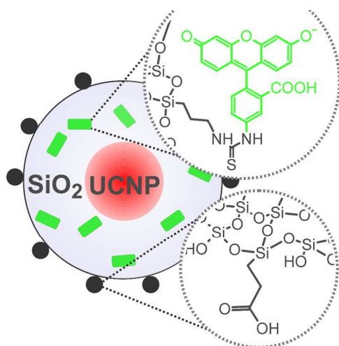
Figure 14 Scheme of silica-coated UCNPs. Fluorescein (green) added during silanization enables the detection in the conventional downconversion mode. Further functionalities (e.g. carboxylic acids) on the surface can be used to improve the water dispersibility of the UCNPs. Reprinted with permission from Ref. 177 Copyright © 2014, American Chemical Society.
