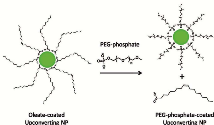
Figure 7 Scheme of the ligand exchange reaction of oleate-coated UCNPs with PEG-phosphate. The hydrophilic PEG-phosphate ligand replaces the hydrophobic oleate ligand by coordinating to the UCNP surface with its phosphate group. Reprinted with permission from Ref. 10. Copyright © 2010 American Chemical Society.
