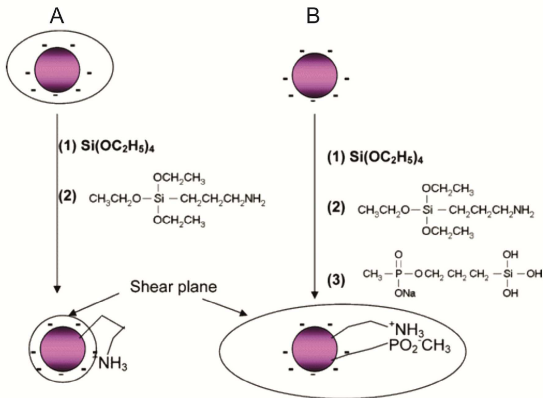
Figure 13 Scheme of the back bonding mechanism of amine-functionalized silica nanoparticles on the same nanoparticle (A) and the potential avoidance by a silanization with methyl phosphonate (B). The simultaneous modification with amines, positively charged at physiological pH, and methyl phosphonate, negatively charged at physiological pH, results in an increased shear plane and electrostatic repulsion. Reprinted with permission from Ref. 161. Copyright © 2006, American Chemical Society.
