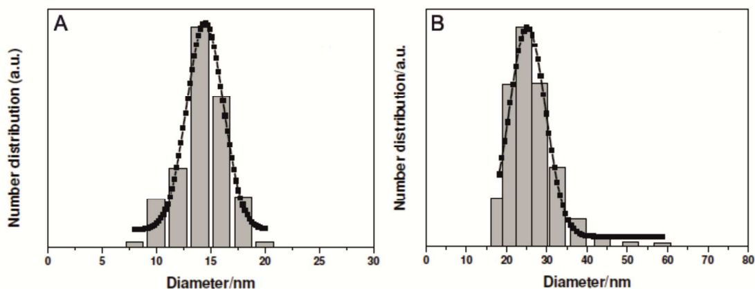
Figure 27 DLS of UCNPs coated with oleylamine (A) and 6-aminohexanoic acid (B). The increase of the hydrodynamic diameter can be attributed to ligand change on the UCNP surface from hydrophobic (low hydrodynamic diameter) to hydrophilic (high hydrodynamic diameter). Also the size distribution remains nearly unaffected indicating a surface modification without aggregation. Reprinted with permission from Ref. 122. Copyright © 2011, American Chemical Society.
