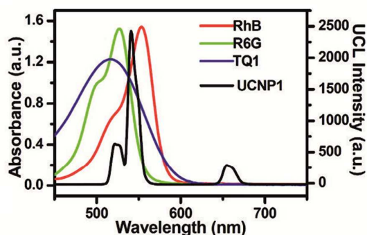
Figure 21 Comparison of the UV-VIS absorption spectra of rhodamine B (RhB), rhodamine 6G (R6G), and Tide Quencher 1 (TQ1) and the emission spectra of NaYF 4 :Yb, Er. The overlapping spectra in the green range enables a luminescence energy transfer (LRET) from the UCNP to the respective dye resulting in a decrease of the green emission of the UCNPs with rising dye concentration and an increase of the dye emission in the case of RhB and R6G. Reprinted with permission from Ref. 138. Copyright © 2011, American Chemical Society.
