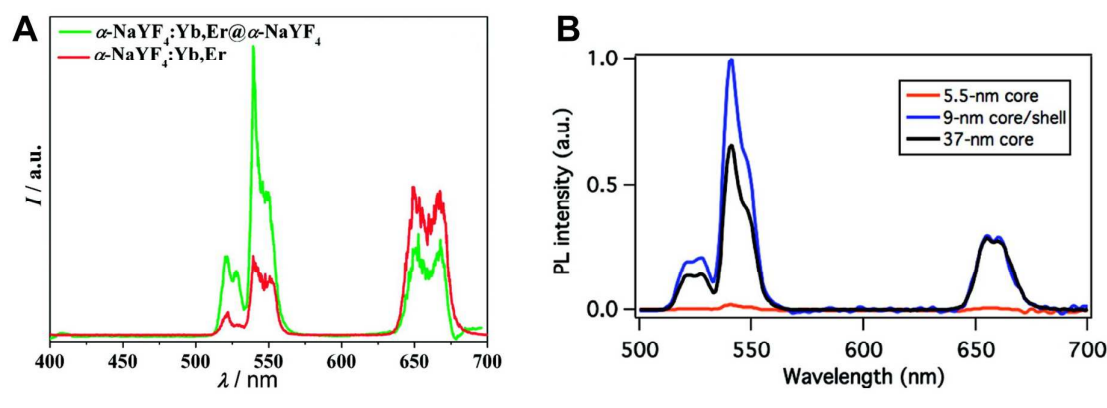
Figure 3 Influence of a core-shell design on the upconversion luminescence of NaYF 4 :Yb,Er nanocrystals under 980-nm excitation. (A) The intensity of the green emission of \alpha -NaYF 4 :Yb 3+ ,Er 3+ @ \alpha -NaYF 4 core/shell nanoparticles increases by a factor of two compared to core-only \alpha -NaYF 4 :Yb 3+ ,Er 3+ . (B) A core/shell design of \beta -NaYF 4 :Yb 3+ ,Er 3+ @NaYF 4 leads to an even stronger luminescence enhancement compared to core-only \beta -NaYF 4 :Yb 3+ ,Er 3+ . Adapted with permission from Ref. 65 and 5. Copyright © 2007 and Copyright © 2012, American Chemical Society.
