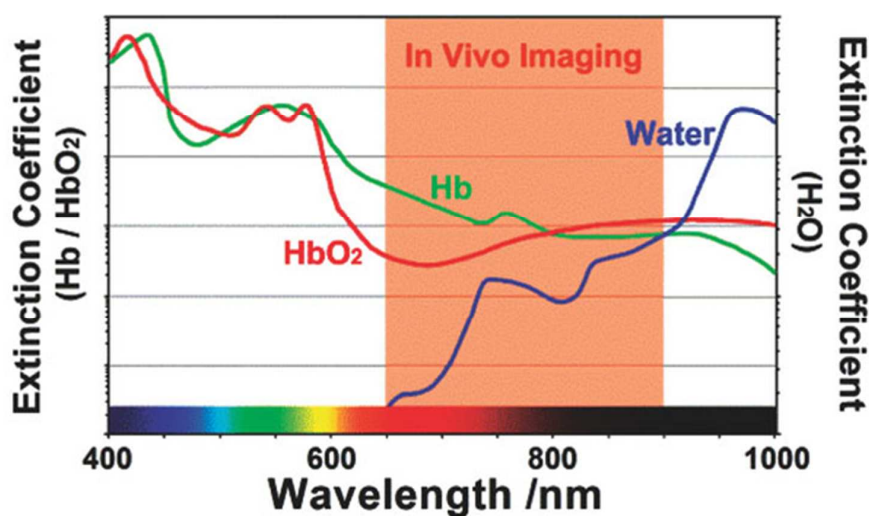
Figure 4 Optimal spectral range for tissue imaging. The absorption of water is 20-fold lower at 800 nm compared to 980 nm. Light absorption of hemoglobin (Hb) and oxyhemoglobin ( \text{HbO}_2 ) can be avoided by using long-wavelength light. Reprinted with permission from Ref. 89 Copyright © 2013, Wiley.
