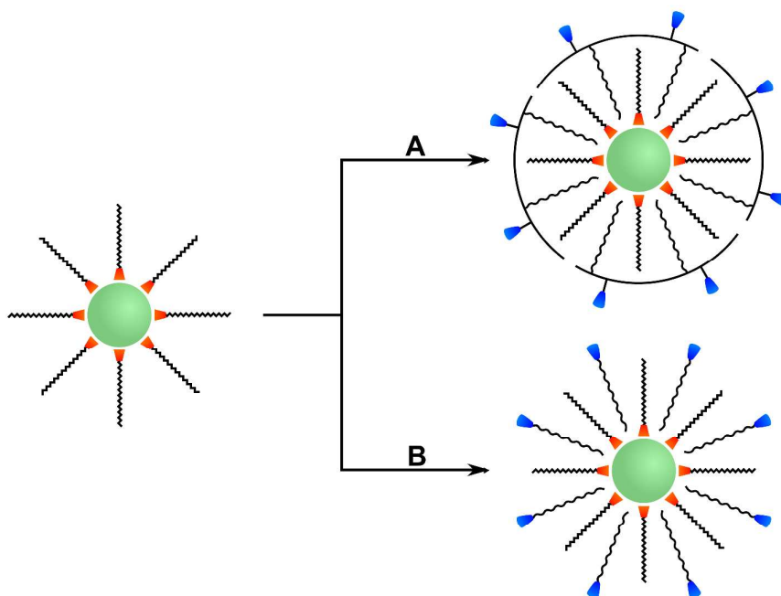
Figure 10 Preparation of functionalized UCNPs by ligand interaction using (A) (modified) polymers with multiple hydrophobic chains to interact with hydrophobic surface and (B) detergents with a single hydrophobic chain.
