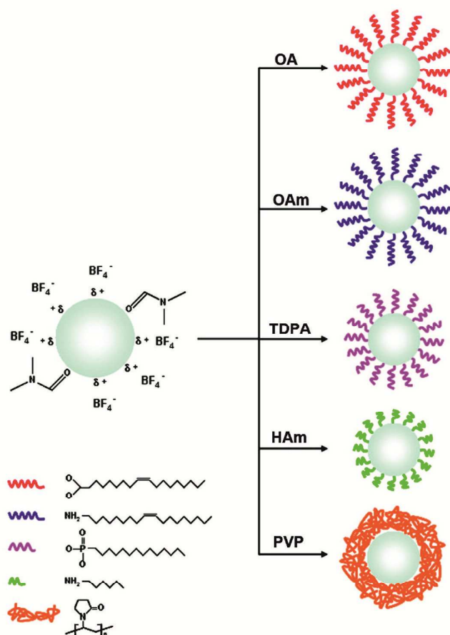
Figure 8 Subsequent ligand exchange reactions of \text{BF}_4^- -coated UCNPs in dimethylformamide (DMF). The use of oleic acid (OA), oleylamine (OAm), tetradecylphosphonic acid (TDPA), or hexylamine (HAm) yields hydrophobic UCNPs dispersible in hexane, while the use of polyvinylpyrrolidone (PVP) results in UCNPs dispersible in aqueous media. Adapted with permission from Ref. 135. Copyright © 2011, American Chemical Society.
