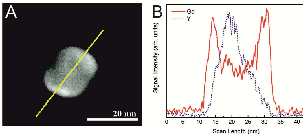
Figure 23 (A) TEM image and (B) EDS scan of a \text{NaYF}_4@ \text{NaGdF}_4 nanoparticle. The yellow line represents the scan line. The EDS scan clearly shows the different material compositions of core and shell. Reprinted with permission from Ref. 67. Copyright © 2011, American Chemical society.
