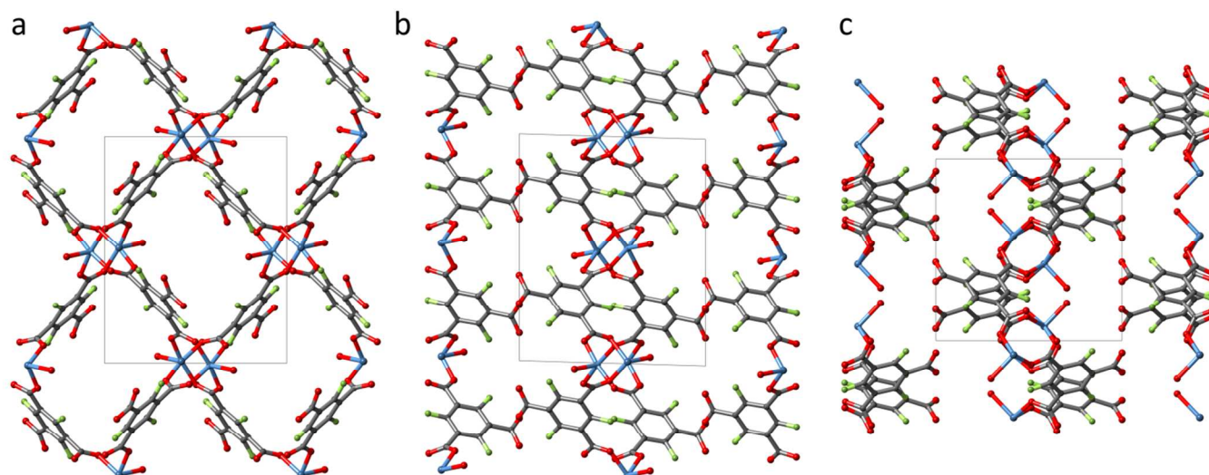
Figure 4: Extended unit cell of UHM-33 along the a -axis (a), the b -axis (b) and the c -axis (c); grey: carbon, red: oxygen, blue: copper, green: fluorine, hydrogen atoms and solvent molecules are omitted for clarity.
