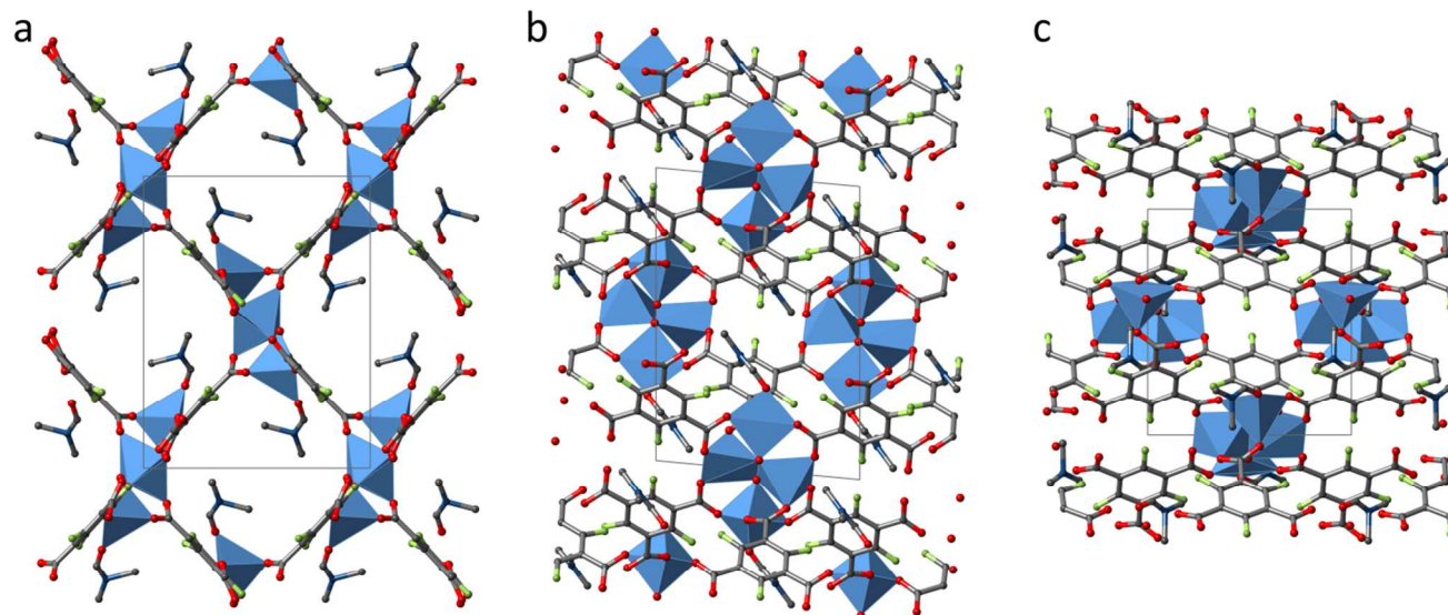
Figure 3: Extended unit cell of UHM-32 along the a -axis (a), the b -axis (b) and the c -axis (c); grey: carbon, red: oxygen, blue: copper, green: fluorine, hydrogen atoms and solvent molecules (apart from the DMA molecules coordinated to the SBU) are omitted for clarity. The coordination spheres of the copper ions are illustrated by the blue polyhedra.
