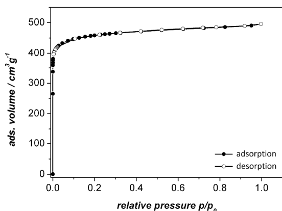
Figure 7: Nitrogen physisorption isotherms of activated UHM-31 measured at 77 K.
