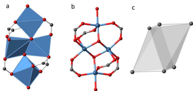
Figure 2: Illustration of the inorganic SBU of UHM-32; grey: carbon, red: oxygen, blue: copper. a: Illustration of the copper coordination sphere in form of the resulting polyhedra, b: Illustration of the connectivity between copper ions and oxygen ions, c: Resulting overall polyhedron built by the points of extension, i.e. the carbon atoms of the carboxyl groups.
