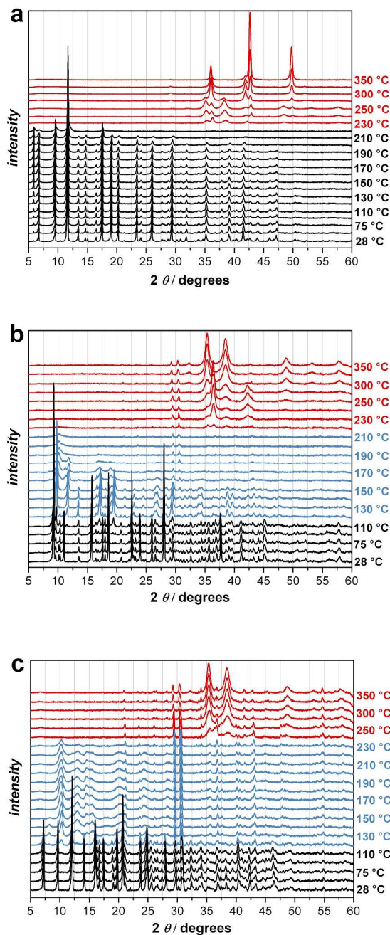
Figure 5: Variable temperature powder XRD pattern of UMH-31 (a), UHM-32 (b) and UHM-33 (c). For each experiment 23 diffractograms were measured, The first three ones at 28, 50 and 75 °C, followed by temperature steps of 10 °C from 100 up to 250 °C and steps of 25 °C up to 350 °C. Black represents the original MOF phase, blue the new MOF phases and red the decomposition products. The two reflections at 2\theta = 29.4 and 2\theta = 30.5 are probably caused by the sample holder.
