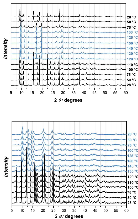
Figure 6: Variable temperature powder XRD patterns of UHM-32 (top) and UHM-33 (bottom). The temperature was increased from 28 °C to 50 °C and 75 °C, than in steps of 10 °C up to 150 °C. The samples were then cooled down to room temperature in steps of 25 °C. Blue represents the new built phases.
