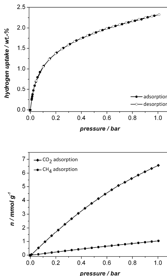
Figure 8: Hydrogen physisorption isotherms measured at 77 K (top) and methane and carbon dioxide physisorption isotherms at 298 K (bottom).
