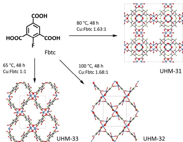
Figure 1: Visualisation and reaction conditions of the three new MOFs that could be synthesised from Fbtc; grey: carbon, red: oxygen, blue: copper, green: fluorine, hydrogen atoms and solvent molecules are omitted for clarity.
