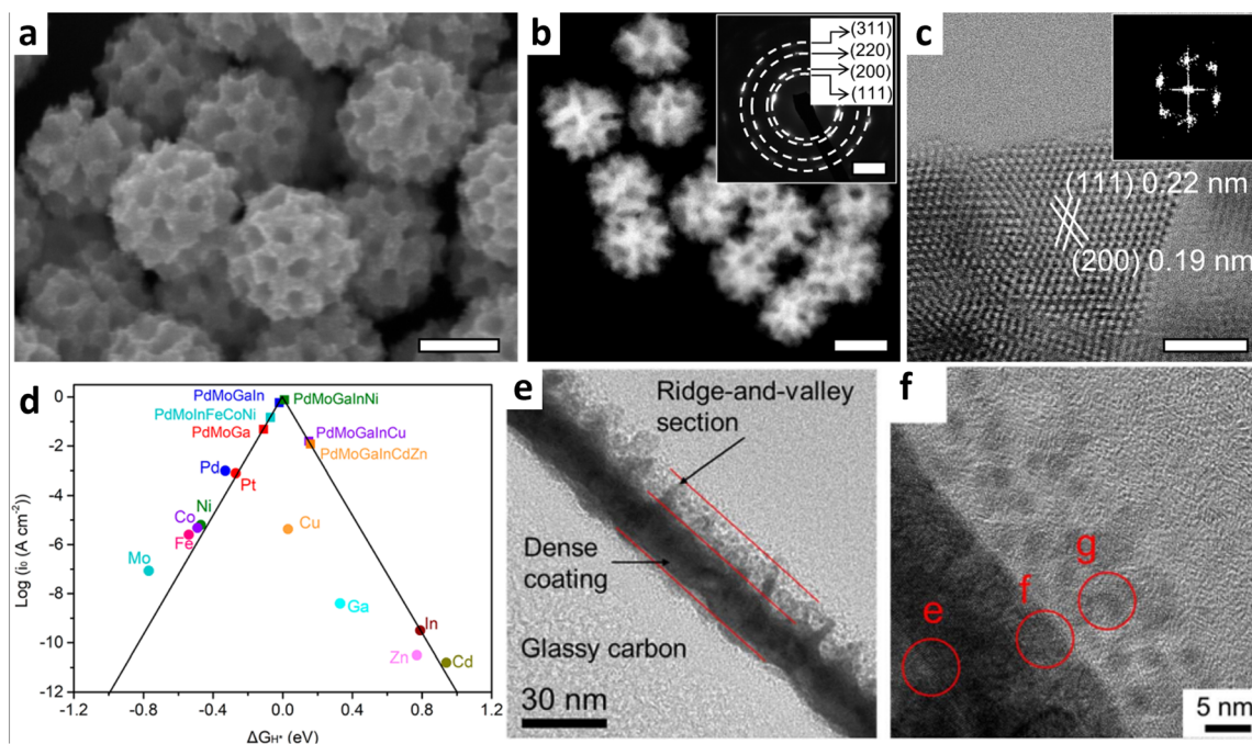
Fig. 9 (a) SEM image (scale bar: 100 nm) and (b) HAADF-STEM image (scale bar: 100 nm). Insets: corresponding SAED patterns (scale bar: 5 nm -1 ). (c) HRTEM (scale bar: 2 nm) (FFT patterns are shown in the inset) of the PtPdRhRuCu mesoporous nanospheres. Reproduced with permission. 62 Copyright 2023, Springer Nature. (d) A plot constructed from experimentally derived exchange current densities and computationally calculated hydrogen binding energies of various single elements and HEAs. Reproduced with permission. 65 Copyright 2022, American Chemical Society. (e) and (f) HR-TEM images of the cross-sectional and subsurface areas of Ir 20.3 Pd 16.3 Pt 8.6 Rh 26.1 Ru 28.7 /GC. Reproduced with permission. 66 Copyright 2024, Royal Society of Chemistry.
