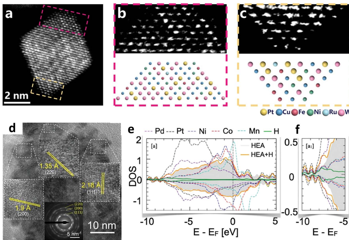
Fig. 7 (a)–(c) HAADF-STEM image and atomically resolved HAADF-STEM images of Ru-doped (0.2 at%) \text{Pt}_{24.8}\text{Fe}_{12.7}\text{Ni}_{7.1}\text{Cu}_{34.5}\text{W}_{20.8} HEA nanocrystals. Corresponding simulated atomic images contained in (b) and (c). Reproduced with permission. 50 Copyright 2024, Wiley-VCH GmbH. (d) HRTEM image showing the d -spacing value of PtPdNiCoMn. (e) and (f) DFT calculation of the PDOS of PtPdNiCoMn and the magnified region. Reproduced with permission. 53 Copyright 2025, Wiley-VCH GmbH.
