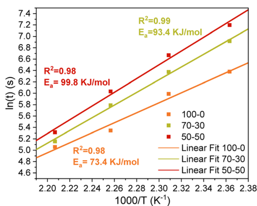
Fig. 9 Linear fitting curves calculated using the Arrhenius equation and activation energies for ECO-ESO samples.
