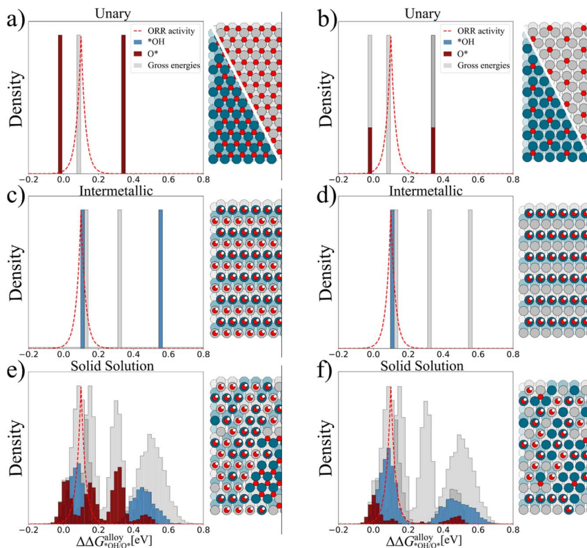
Fig. 5 Left column shows gross (grey background) and net (full colour) *OH/O* adsorption energy distributions and illustration of the adsorbate coverage when the adsorbates are blocking according to the mutual blocking rules for (a) unary Pd(111) or Ag(111), (c) intermetallic PdAg(111), and (e) equimolar solid solution PdAg(111). Right column shows gross (grey background) and net (full colour) *OH/O* adsorption energy distributions and illustration of the adsorbate coverage when the adsorbates are blocking in accordance with the extended blocking scheme for (b) unary Pd(111) or Ag(111), (d) intermetallic PdAg(111), and (f) equimolar solid solution PdAg(111).
