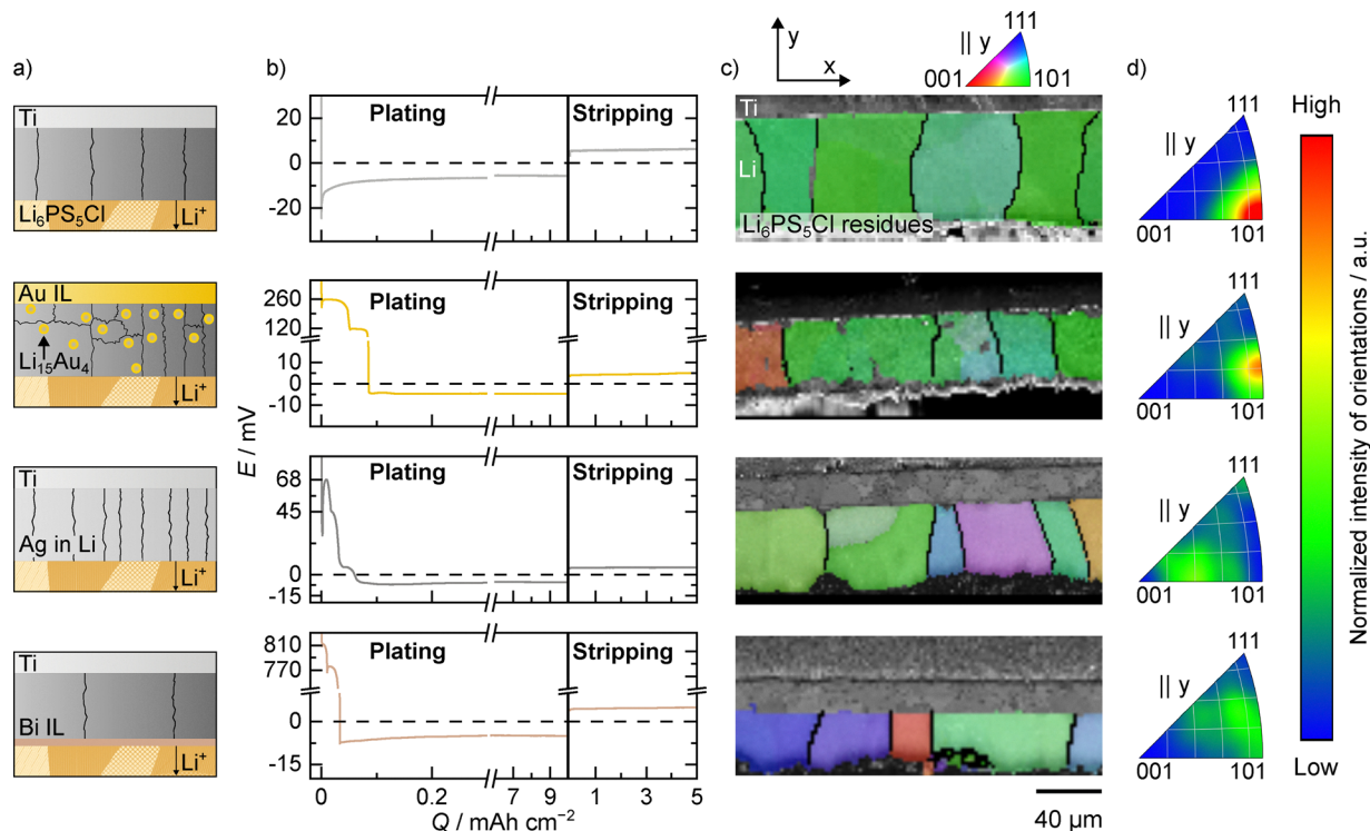
Fig. 4 Microstructure of electrodeposited lithium after stripping. (a) Cell setup used for stripping after electrodeposition of 10 \text{ mAh cm}^{-2} of lithium. The location of the interlayers is indicated schematically. (b) Potential profile during electrodeposition of 10 \text{ mAh cm}^{-2} lithium on the left and subsequent stripping of 5 \text{ mAh cm}^{-2} on the right. (c) Microstructure of the partially stripped lithium layers using the different interlayer materials. The IPF maps are given parallel to the y -direction as indicated above. The shown scalebar resembles 40 \mu\text{m} in all cases. (d) IPFs of the partially stripped lithium layers, showing the distribution of all measured grain orientations. Please note that the IPFs were created based on the entire analyzed cross-section, which is shown in the SI.
