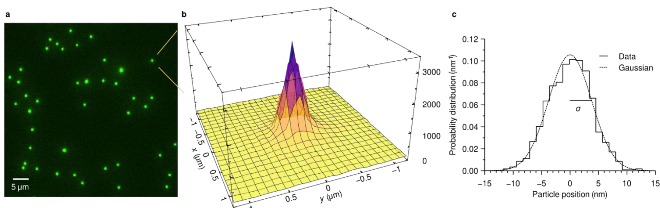
Figure 1. Localisation precision of particles adhering to glass. a , Widefield fluorescence image of 200 nm diameter particles adhering to glass. b , Fluorescence intensity distribution of the particle indicated in panel a. The size of the grid is given by the size of a
