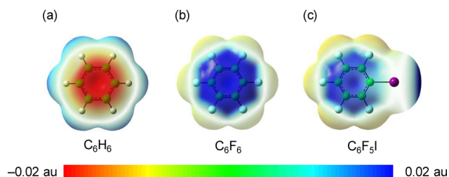
Fig. 1 Electrostatic potential maps of (a) benzene, (b) perfluorobenzene (C 6 F 6 ), and (c) pentafluoriodobenzene (C 6 F 5 I).
