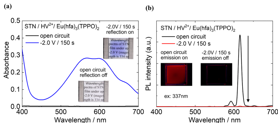
Fig. 6 (a) Absorption spectra of the STN/HV 2+ /Eu(hfa) 3 (TPPO) 2 film under open circuit condition (black line) and applied -2.0 \text{ V} for 150 \text{ s} (blue line). (b) Emission spectra of the STN/HV 2+ /Eu(hfa) 3 (TPPO) 2 film under open circuit condition (black line) and applied -2.0 \text{ V} for 150 \text{ s} (red line). Excitation wavelength is 337 \text{ nm} .
