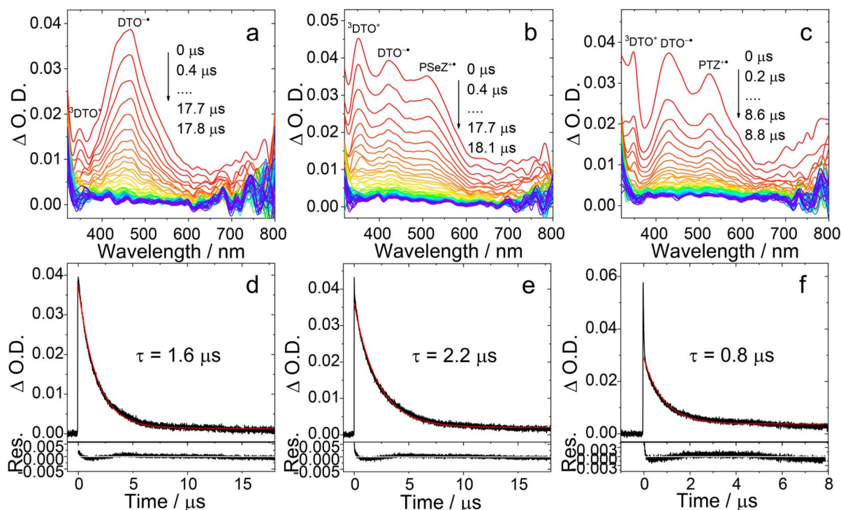
Fig. 6 Nanosecond transient absorption spectra of (a) PTZ-DTO, (b) PSeZ-DTO and (c) DPTZ-DTO. Decay curves of (d) PTZ-DTO, (e) PSeZ-DTO at 460 nm and (f) DPTZ-DTO at 530 nm after pulsed laser excitation at 355 nm. c = 2.0 \times 10^{-5} M in deaerated TOL, 25 °C.
