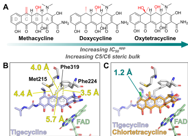
Fig. 4 Increasing C5 and C6 steric bulk of tetracyclines results in weaker affinity, offering a strategy for development of tetracyclines that evade Tet(X) resistance. (A) Structure of C5- and C6-substituted tetracyclines tested in this study. (B) Distance measurements between C5/C6 of tigecycline and nearby active site residues (PDB: 7EPW). 8 (C) Displacement of chlortetracycline, a C6-substituted tetracycline, in complex with Tet(X2) relative to tigecycline (PDB: 2Y6R). 46 This displacement is likely necessary to avoid steric clashes of the C6-substitutions with active site residues. Superimposition of structures was performed in PyMOL v2.5.0 (Schrödinger, LLC).
