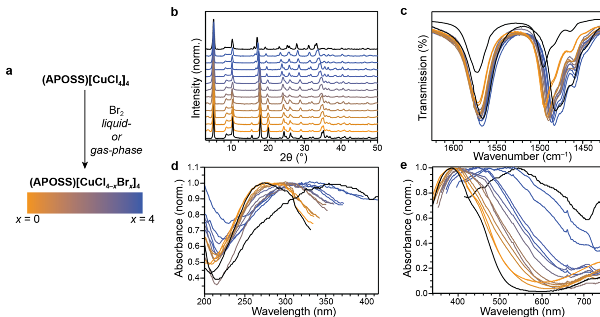
Fig. 3 (a) Scheme of post-synthetic halide exchange using Br 2 , either in the liquid or gas phase. The specific bromide content, as determined by EDX, for these 14 samples are 0.0, 5.8, 10.4, 11.0, 21.7, 27.8, 39.5, 42.3, 43.3, 55.8, 59.2, 79.8, 90.0, and 100.0% (expressed as a gradient). Black lines on either side represent x = 0 or x = 4 . (b) Powder X-ray diffraction patterns for (APOSS)[CuCl 4-x Br x ] 4 . (c) Infrared spectra of (APOSS)[CuCl 4-x Br x ] 4 , highlighting the symmetric N–H vibration around 1490 cm -1 . (d and e) Diffuse reflectance spectra of (APOSS)[CuCl 4-x Br x ] 4 , highlighting two LMCT transitions.
