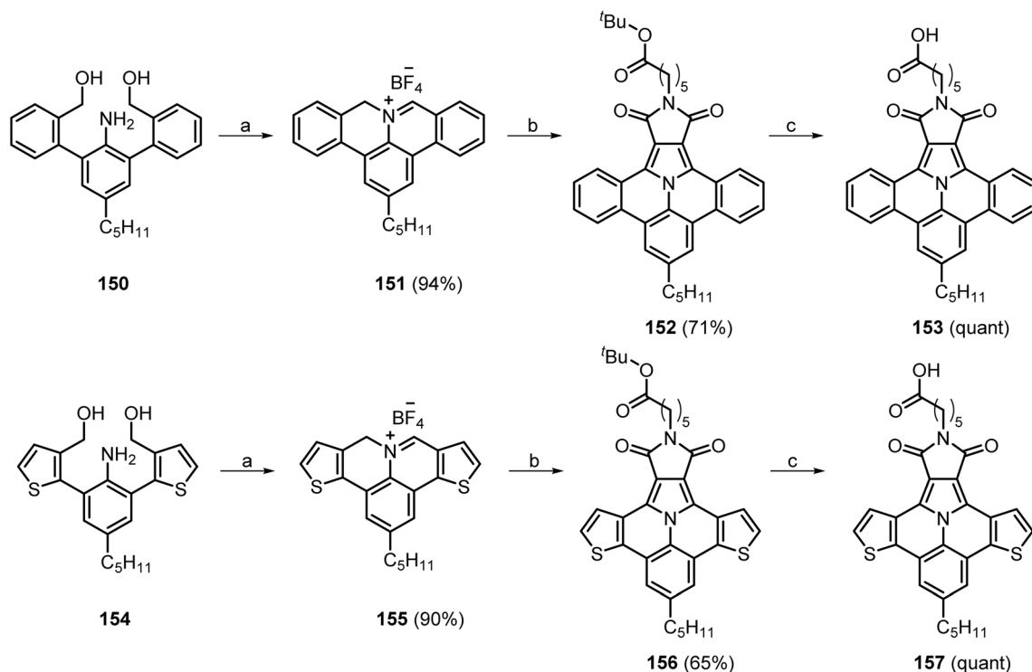
Scheme 40 Synthesis of supramolecular polymer scaffolds. Conditions: (a) (step i) HCl (4 M in 1,4-dioxane), MW, 130 °C, \text{N}_2 ; (step ii) \text{CPh}_3\text{BF}_4 , \text{CH}_3\text{CN}/\text{toluene} , 90 °C, \text{N}_2 ; (b) (step i) tert butyl 6-maleimidohehexanoate, \text{Et}_3\text{N} , \text{CH}_2\text{Cl}_2 , 25 °C, \text{N}_2 ; (step ii) DDQ, \text{CH}_2\text{Cl}_2/\text{toluene} , 25 °C, \text{N}_2 ; (c) \text{CF}_3\text{CO}_2\text{H} , \text{CH}_2\text{Cl}_2 , 25 °C.
