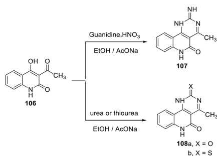
Scheme 56 Synthesis of pyrimido[5,4- c ]quinolines 107 and 108a,b from 3-acyl-4-hydroxy-quinoline-2-one ( 106 ).
