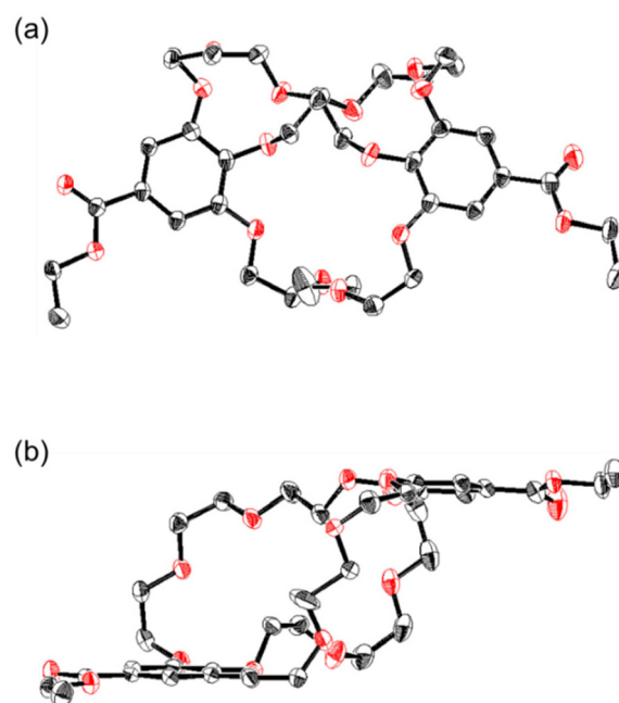
Fig. 6 ORTEP representation of the solid-state structure of cryptand 1a . (a) Overhead view and (b) side view. Thermal ellipsoids are shown at the 50% probability level. For clarity, hydrogen atoms and disordered oxyethylene chains are omitted. Black: carbon; red: oxygen.
