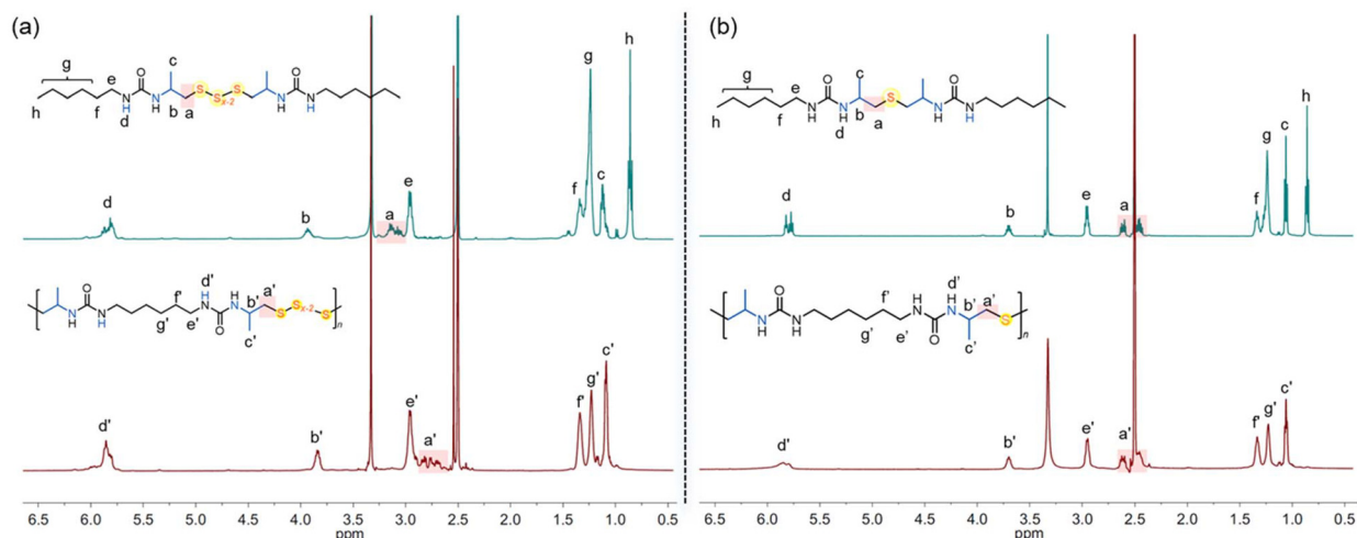
Fig. 1 1 H NMR spectra of (a) UA1-S x and PUA1-S x , and (b) UA1-S and PUA1-S.
