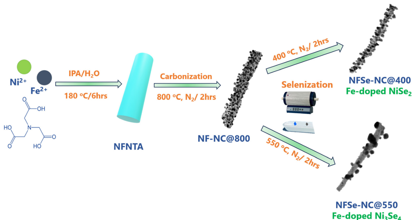
Fig. 1 Schematic representation of the synthesis of Ni x Fe 1-x Se 2 -NC@400 and Ni 3-x Fe x Se 4 -NC@550.
