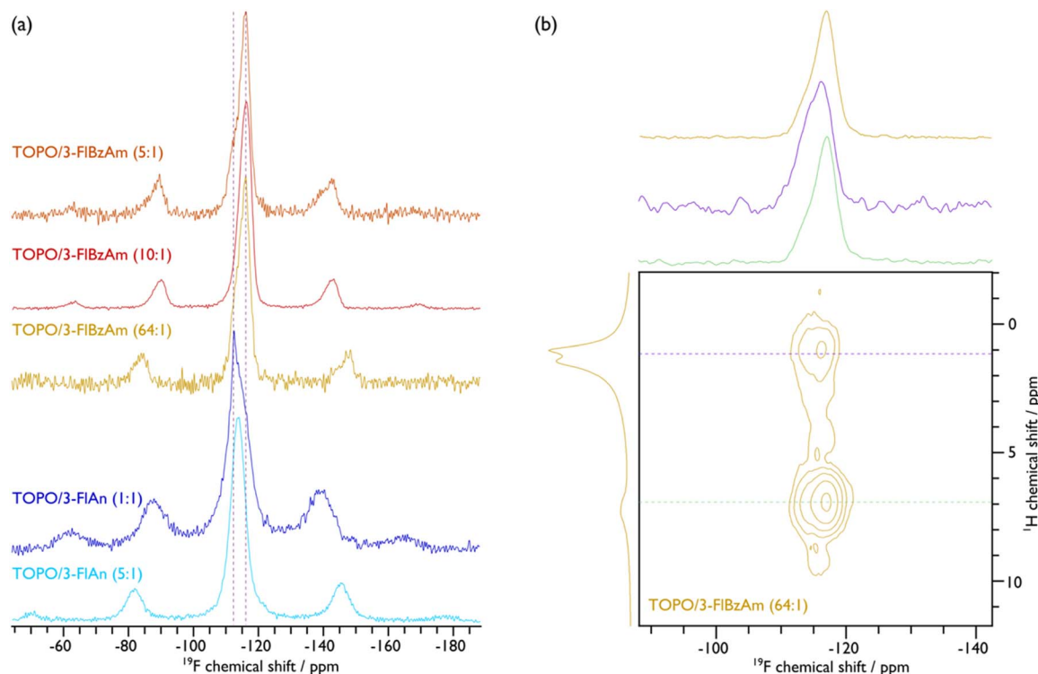
Fig. 5 \{^1\text{H}-^{19}\text{F}\} CP (a) and ^1\text{H}-^{19}\text{F} 2D dipolar correlation (b) MAS NMR spectra of indicated CdS NCs. An MAS frequency of 10 kHz was used for TOPO/3-FlAn (1 : 1), TOPO/3-FIBzAm (10 : 1), and TOPO/3-FIBzAm (5 : 1), and 12 kHz was used for TOPO/3-FlAn (5 : 1) and TOPO/3-FIBzAm (64 : 1) CdS NCs. Cross-sectional slices at the positions indicated with the horizontal dashed coloured lines in the 2D spectrum are given above the 2D spectrum in (b) along with the corresponding \{^1\text{H}-^{19}\text{F}\} CP (top) and ^1\text{H} (left) MAS NMR spectra. See the ESI† for corresponding spectral fittings.
