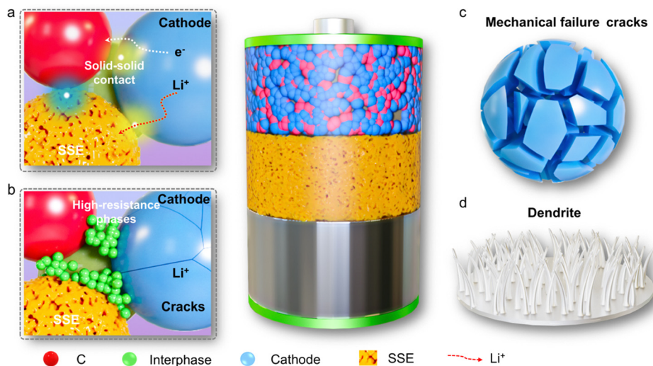
Fig. 11 Schematic diagram of solid electrode–electrolyte interface problems.
