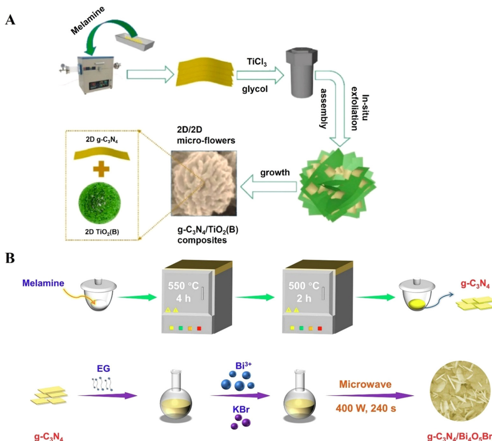
Fig. 5 (A) Schematic synthesis procedure of the g-C 3 N 4 /TiO 2 (B) covalent heterojunction, reproduced with permission from ref. 91, and (B) the g-C 3 N 4 /Bi 4 O 5 Br 2 noncovalent heterojunction, reproduced with permission from ref. 92.
