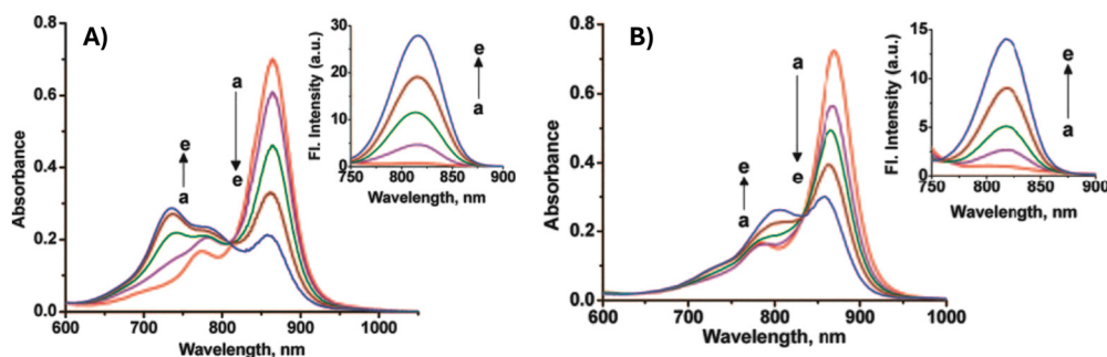
Fig. 16 Changes in the absorption spectra of CR47a (7.75 μM) in THF with addition of (A) Pb^{2+} [ Pb^{2+} ] = 0 (a), 0.94 (b), 1.88 (c), 2–82 (d) and 3.87 μM (e) and (B) Cd^{2+} [ Cd^{2+} ] = 0 (a), 0.94 (b), 1.88 (c), 2–82 (d) and 3.87 μM (e). The insets show the corresponding changes in fluorescence intensity. Excitation wavelength = 700 nm. Reproduced with permission from ref. 23. Copyright 2008, the American Chemical Society.
