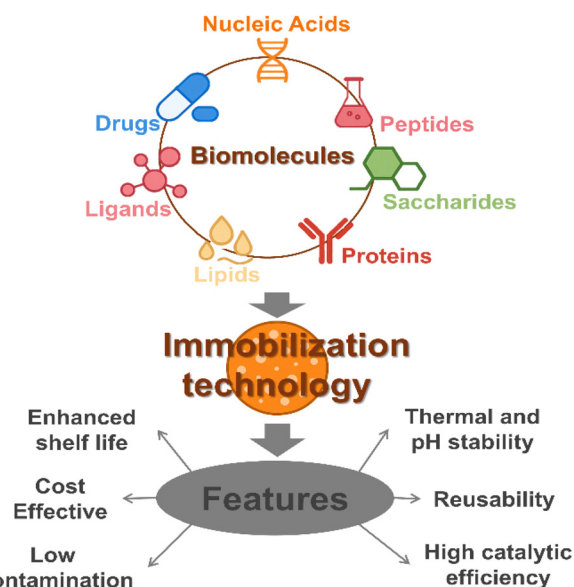
Fig. 7 Major classes of biomolecules commonly immobilized and their typical applications.
