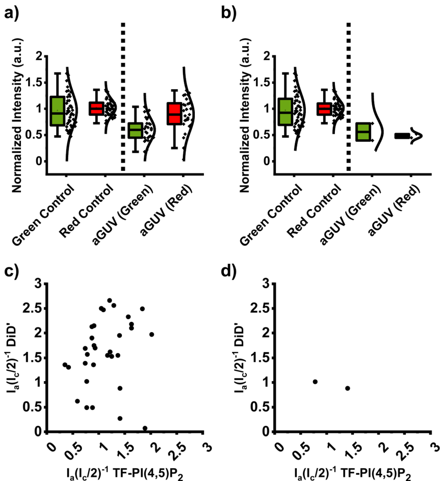
Fig. 3 DOPC/DiD (inner leaflet, red channel): DOPC/PI(4,5) \text{P}_2 /TF-PI(4,5) \text{P}_2 (outer leaflet, green channel) asymmetric giant unilamellar vesicles prepared using 6 mM \text{Ca}^{2+} as the hemifusion initiator. (a) Comparison of sGUV controls for the green (DOPC/PI(4,5) \text{P}_2 /TF-PI(4,5) \text{P}_2 ; N = 51 ) and red (DOPC/DiD'; N = 47 ) channels to the corresponding fluorescence channels of imaged aGUVs ( N = 32 ) across 6 separate experiments. (b) The range-passing aGUVs (see text) from the samples presented in panel A. (c) Cross-correlation of the two channels for individual aGUVs. A "perfect" aGUV would be found at the data point (1,1) which corresponds to a completely exchanged outer leaflet and no artifacts like multi-lamellarity. (d) Cross-correlation of the two channels for the range-passing aGUVs. sGUV buffer: 97 mM NaCl, 100 mM KCl, 1 mM \text{Na}_2\text{EDTA} , 25 mM HEPES pH = 7.4 buffer. aGUV buffer after hemifusion: 97 mM NaCl, 100 mM KCl, 7 mM \text{Na}_2\text{EDTA} , 25 mM HEPES pH = 7.4 buffer. The controls displayed in (a) and (b) are the same experiments and are reproduced for comparison.
