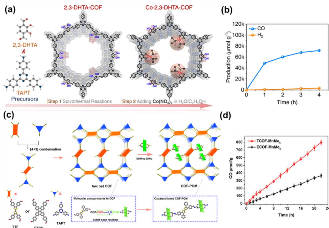
Fig. 11 (a) Synthesis of 2,3-DHTA-COF and Co-2,3-DHTA-COF. (b) CO and \text{H}_2 evolution with irradiation time for the \text{CO}_2 RR catalyzed by Co-2,3-DHTA-COF under visible light irradiation. Adapted with permission. 111 Copyright 2023, Springer Nature. (c) Schematic of uniformly dispersed POM clusters in the COF by confining them into the pores of the COF through covalent linkages. (d) Time-dependent \text{CO}_2 -to-CO performance for TCOF- \text{MnMo}_6 and ECOF- \text{MnMo}_6 . Reproduced with permission. 119 Copyright 2022, American Chemical Society.
