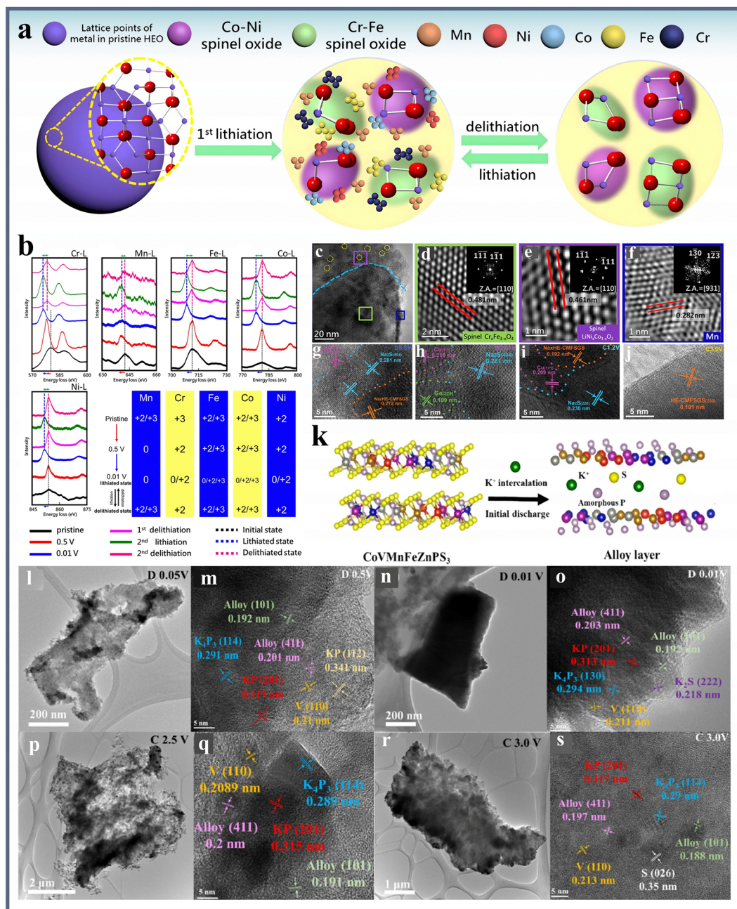
Fig. 2 (a) Lithiation/delithiation processes in (CrMnFeCoNi) 3 O 4 , and (b) EELS L-edge spectra of Cr, Mn, Fe, Co, and Ni elements and summary of valence state variations of constituent elements of HEO. (c) TEM and HRTEM images of (d) Cr x Fe 3-x O 4 , (e) LiNi x Co 1-x O 2 , and (f) Mn phases of (CrMnFeCoNi) 3 O 4 . Reproduced with permission. 31 Copyright 2021, Elsevier Inc. Ex situ TEM patterns under sodiation conditions of CuMnFeSnGeS at (g) 0.6 V and (h) 0.01 V and desodiation states of (i) 1.2 V and (j) 3.0 V. Reproduced with permission. 32 Copyright 2022, Wiley-VCH. (k) Schematic illustration of the K + storage mechanism CoVMnFeZnPS 3 during the charging/discharging process. Low magnification TEM images of the cycled CoVMnFeZnPS 3 : (l) and (m) discharged to 0.5 V, (n) and (o) discharged to 0.01 V, (p) and (q) charged to 2.5 V, and (r) and (s) charged to 3.0 V. Reproduced with permission. 33 Copyright 2023, Elsevier Inc.
