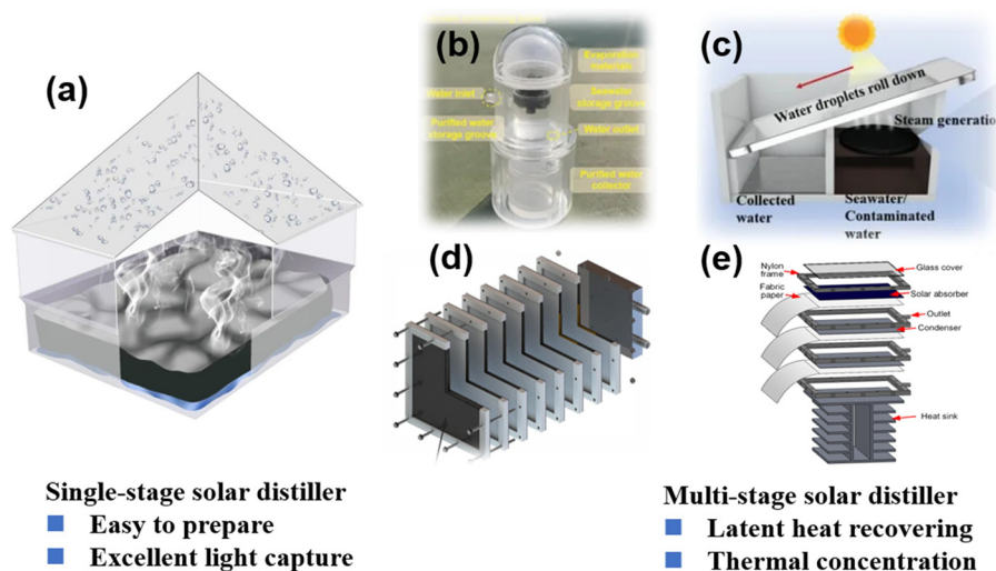
Single-stage solar distiller ■ Easy to prepare ■ Excellent light capture Multi-stage solar distiller ■ Latent heat recovering ■ Thermal concentration Fig. 20 Fundamental design principles of single-stage and multi-stage solar distillers. (a) Schematic diagram of a vapor condensation device. (b) Vapor upward condensation and collection devices (single stage). Reproduced with permission. 165 Copyright 2024, Wiley-VCH; (c) water droplets collection device (single stage). Reproduced with permission. 166 Copyright 2023, Wiley-VCH; (d) and (e) vapor downward condensation device. (d) Reproduced with permission. 167 Copyright 2024, Springer Nature; (e) reproduced with permission. 63 Copyright 2024, Royal Society of Chemistry.
