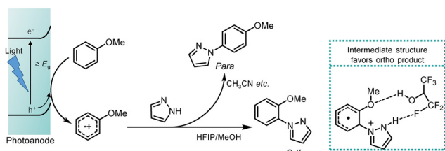
Fig. 10 Proposed mechanism for photoelectrocatalytic C–N coupling of anisole with pyrazole, and the green dotted square includes the proposed hydrogen bonding among anisole, pyrazole, and hexafluoroisopropanol (solvent), which may contribute to the favorable formation of the ortho product. Reproduced from ref. 64, with permission from Springer-Nature, copyright 2019.
