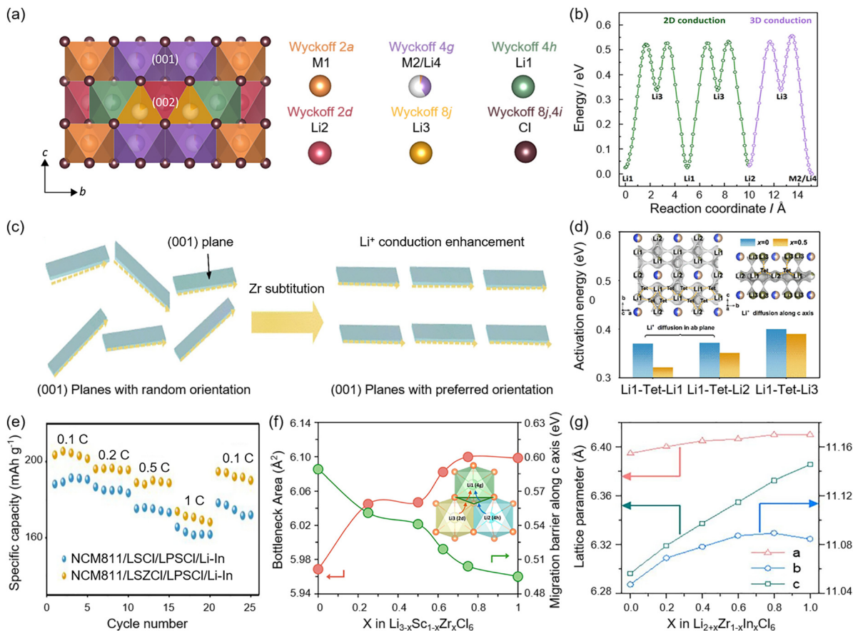
Fig. 6 Cation site distribution and migration pathway affected by aliovalent substitution. (a) Crystal structure of Li 3 InCl 6 . (b) Optimal Li + diffusion pathway from bond valence sum calculations. Reproduced with permissions from ref. 78. Copyright 2021, American Chemical Society. (c) Schematic illustration of Zr 4+ substitution changing the (001) plane preferred orientation. (d) Comparison of activation energy through different migration pathways before and after Zr 4+ doping. (e) Rate capability of batteries after Zr 4+ doping. Reproduced with permissions from ref. 92. Copyright 2022, Elsevier. (f) Change in the bottleneck area and migration barrier for Li + diffusion along the c-axis. The inset depicts the bottleneck area for Li + migration along the c-axis. Reproduced with permissions from ref. 93. Copyright 2024, American Chemical Society. (g) Correlation curves of lattice parameter with In 3+ doping amount. Reproduced with permissions from ref. 94. Copyright 2022, Elsevier.
