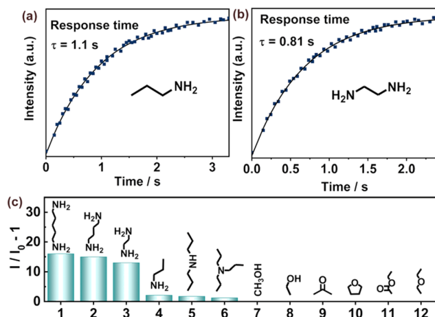
Fig. 6 (a) Response time and time-resolved emission of \text{Eu}_4\text{L}_4.4 before and after the addition of PA; (b) response time and time-resolved emission of \text{Eu}_4\text{L}_4.4 before and after the introduction of EDA; and (c) emission changes of \text{Eu}_4\text{L}_4.4 upon adding various biogenic amines and O-containing compounds.
