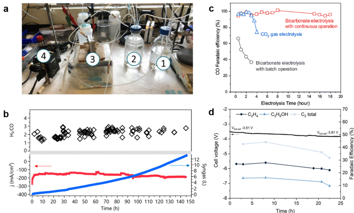
Fig. 18 Stability evaluation of the integrated \text{CO}_2 capture and electrochemical conversion. (a) Experimental setup, where \text{CO}_2 is captured into 2 M KOH (1) to generate carbonate, which is then pumped into a new bottle (2) and reduced in a direct carbonate cell (3). The gas products are measured by a mass flow meter (4) to determine the total volume. (b) Syngas production performance during electrolysis at a constant potential of 3.8 V using a Ag catalyst with the same experimental setup. Reproduced with permission from ref. 72. (c) Stability comparison of electrolysis between gas-fed \text{CO}_2 and 3 M \text{KHCO}_3 with/without \text{CO}_2 purging at a constant current density of 200 \text{ mA cm}^{-2} using a Ni SAC. Reproduced with permission from ref. 90. (d) Long-term operation for \text{CO}_2 capture and electrolysis in a 2 M KOH solution, performed with a Cu/CoPc-CNTs electrocatalyst and a 135 mm MEC interposer. Reproduced with permission from ref. 103.
