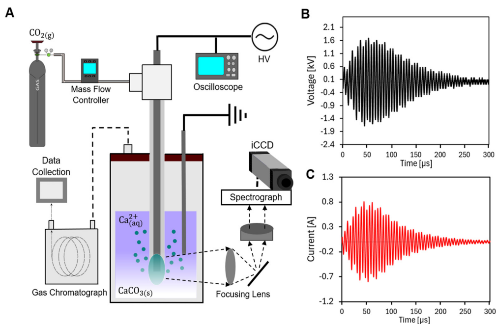
Fig. 1 Experimental overview and pulse plasma discharge characteristics. (A) An experimental schematic of the plasma bubble reactor for CO 2 mineralization to CaCO 3 . (B) and (C) Example of nanosecond pulse voltage–current waveforms taken for the carbonation experiment where the frequency is 500 Hz, the duty cycle is 83 μs, and the resonance frequency is 60.00 kHz (CO 2 flow rate: 200 sccm). Solution conditions: 0.500 M CaCl 2 and 0.750 M NH 4 OH in deionized (D.I.) water.
