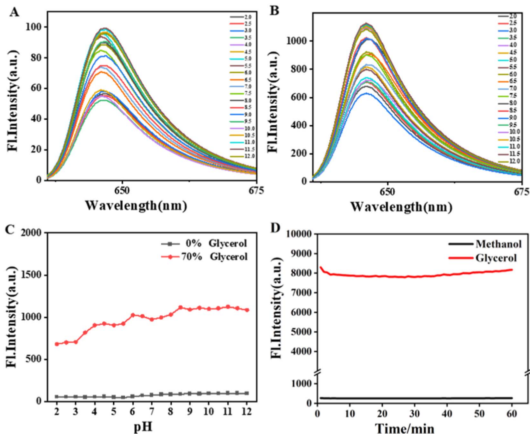
Fig. 6 (A) Fluorescence signal of LTP-H (10 \mu\text{M} ) in a pH-buffer liquid system of pure methanol. (B) Fluorescence signal of LTP-H (10 \mu\text{M} ) in a pH-buffer liquid system with 70% glycerol. (C) Fluorescence signal of LTP-H (10 \mu\text{M} ) in pH systems with different viscosities. (D) Photostability of LTP-H (10 \mu\text{M} ) under constant laser exposure in glycerol and methanol (60 min). \lambda_{\text{ex}} = 570 \text{ nm} , \lambda_{\text{em}} = 650 \text{ nm} .
