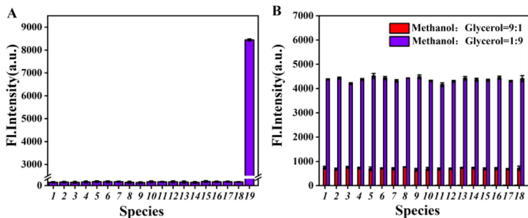
Fig. 5 (A) Selectivity experiments with the probe LTP-H (10 \mu\text{M} ). (B) Fluorescence spectrum of LTP-H (10 \mu\text{M} ) with the addition of analytes in two viscosity systems (fluorescence intensity at 650 nm). (1) Blank. (2) \text{Fe}^{2+} . (3) \text{Fe}^{3+} . (4) \text{Co}^{2+} . (5) \text{Hg}^+ . (6) \text{Ca}^{2+} . (7) \text{Mg}^{2+} . (8) \text{F}^- . (9) \text{SCN}^- . (10) \text{H}_2\text{PO}_4^- . (11) \text{SO}_4^{2-} . (12) \text{CO}_3^{2-} . (13) \text{ONOO}^- . (14) \text{HClO} . (15) \text{HSO}_3^- . (16) \text{S}_2\text{O}_3^{2-} . (17) Hcy. (18) Ser. (19) Glycerol. \lambda_{\text{ex}} = 570 \text{ nm} , \lambda_{\text{em}} = 650 \text{ nm} .
