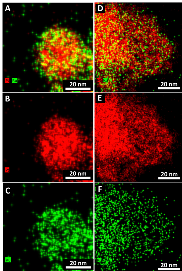
Fig. 2 EDS elemental maps of PtRu generated using the CTAB method. Pt 1 Ru 1 maps are provided as follows: (A) the composite of Pt and Ru, (B) Pt, and (C) Ru. Analogous Pt 3 Ru 1 maps are shown, as (D) the composite of Pt and Ru, (E) Pt, and (F) Ru.
