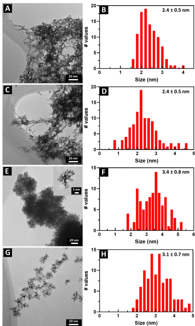
Fig. 1 TEM images and size distributions are shown of a range of chemically distinctive ultrathin NWs, prepared by different synthesis methods. (A) and (B) Pt 1 Ru 1 and (C) and (D) Pt 3 Ru 1 were both prepared with CTAB. (E) and (F) Pt 1 Ru 1 with the inset showing an individual cluster as well as (G) and (H) Pt 1 Ru 9 were generated with OAm and OA.
