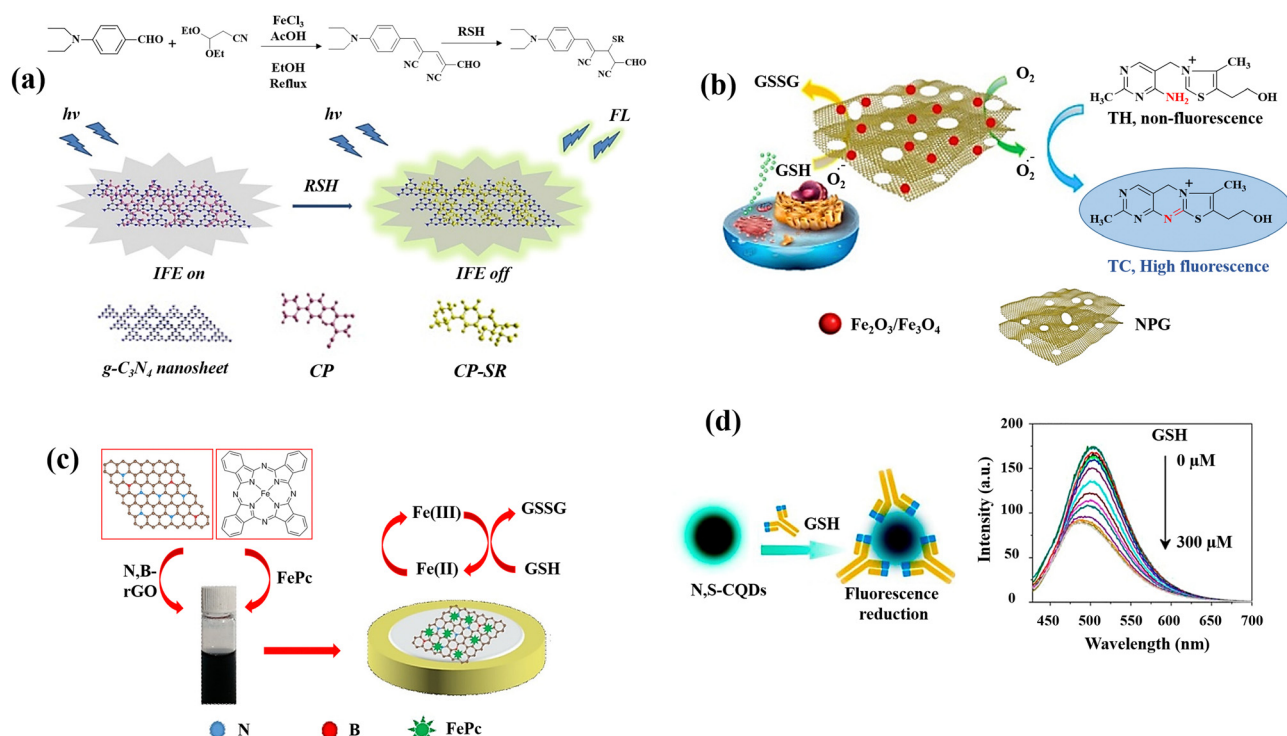
Fig. 2 Schematic illustration of GSH detection with carbon-based nanomaterials: (a) the IFE-based fluorescence sensor g\text{-C}_3\text{N}_4 nanosheets/CP, 42 (b) the MNPNG-based fluorescent assay, 44 (c) the FePc/N,B-rGO nanocomposite, 46 and (d) graphical example of the N,S-CQDs fluorescence response to GSH along with the fluorescence spectra of N,S-CQDs combined with different levels GSH 47 reproduced with the permission of Elsevier and American Chemical Society.
