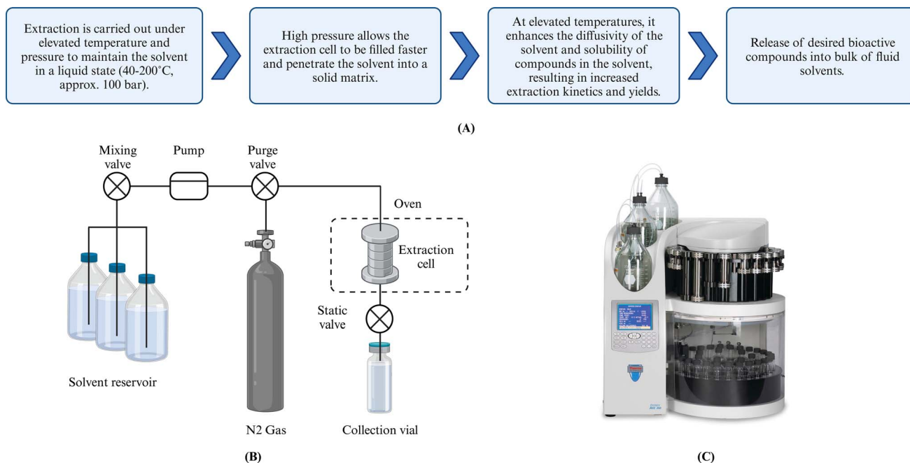
Fig. 3 (A) Mechanism of ASE technique. (B) Schematic of the ASE Process. (C) Commercial automated accelerated solvent extractor. Created with https://www.biorender.com/ .
