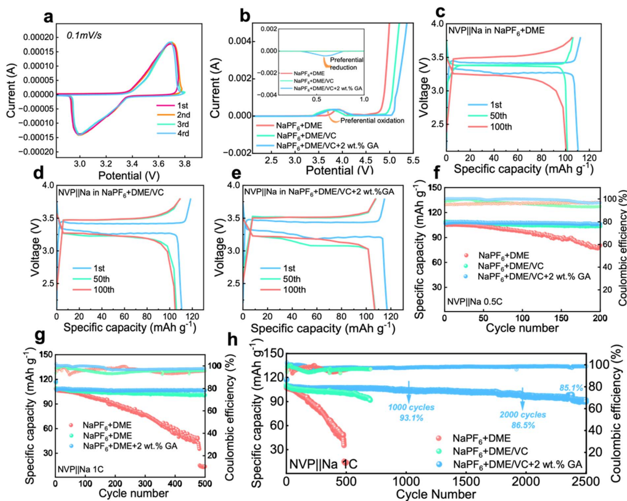
Fig. 3 The electrochemical performance of electrolytes. (a) The 1st–4th CV curves of the \text{Na}||\text{NVP} battery in the electrolyte containing 2 wt% GA additive. (b) The LSV curves of the \text{Na}||\text{NVP} battery in the three electrolytes. (c–e) The corresponding galvanostatic charge/discharge curves of the three \text{Na}||\text{NVP} batteries at different cycles. The cycle performance of \text{Na}||\text{NVP} batteries in different electrolytes (f) for 200 cycles at 0.5C and (g) for 500 cycles at 1C and (h) for 2500 cycles at 1C.
